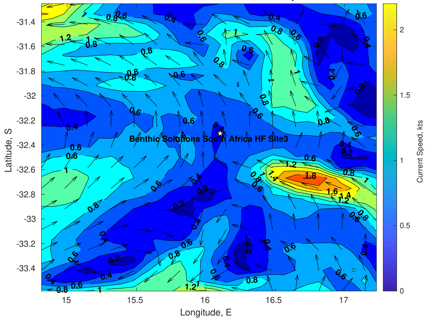
Surface Currents for Benthic Solutions South Africa HF Site3 at 13-May-2025 00:00:00
