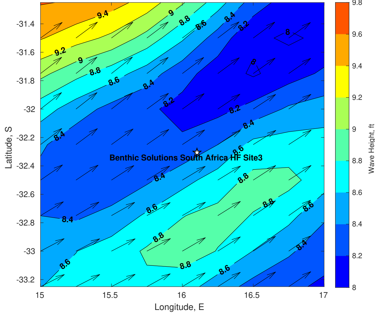
Wave Height (ft) for Benthic Solutions South Africa HF Site3 at 14-May-2025 09:00:00
