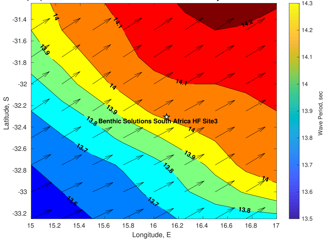
Wave Period (sec) for Benthic Solutions South Africa HF Site3 at 14-May-2025 09:00:00
