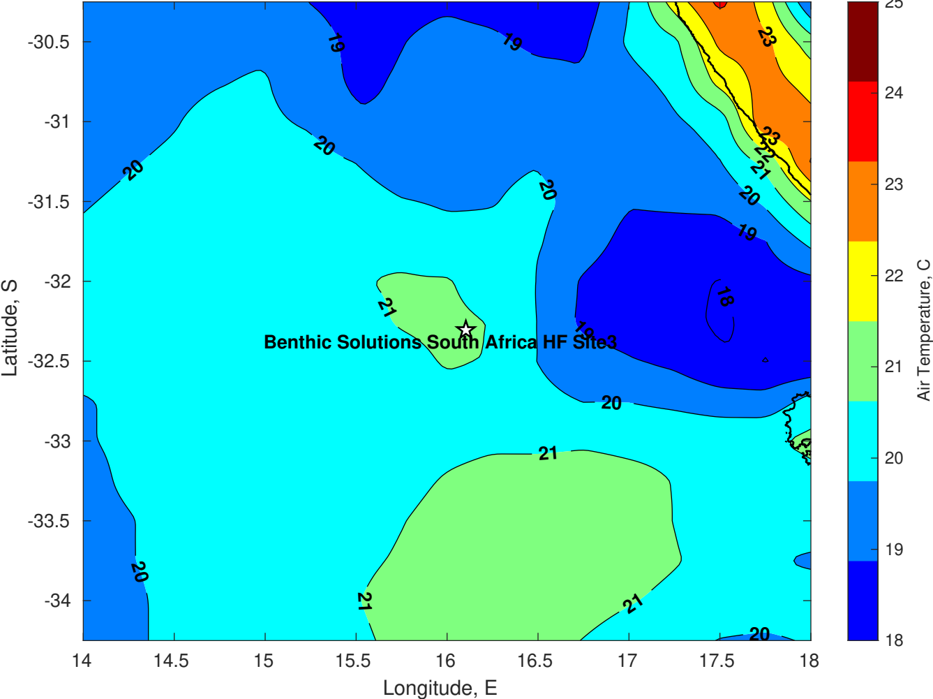
Air Temperature (C) for Benthic Solutions South Africa HF Site3 at 14-May-2025
