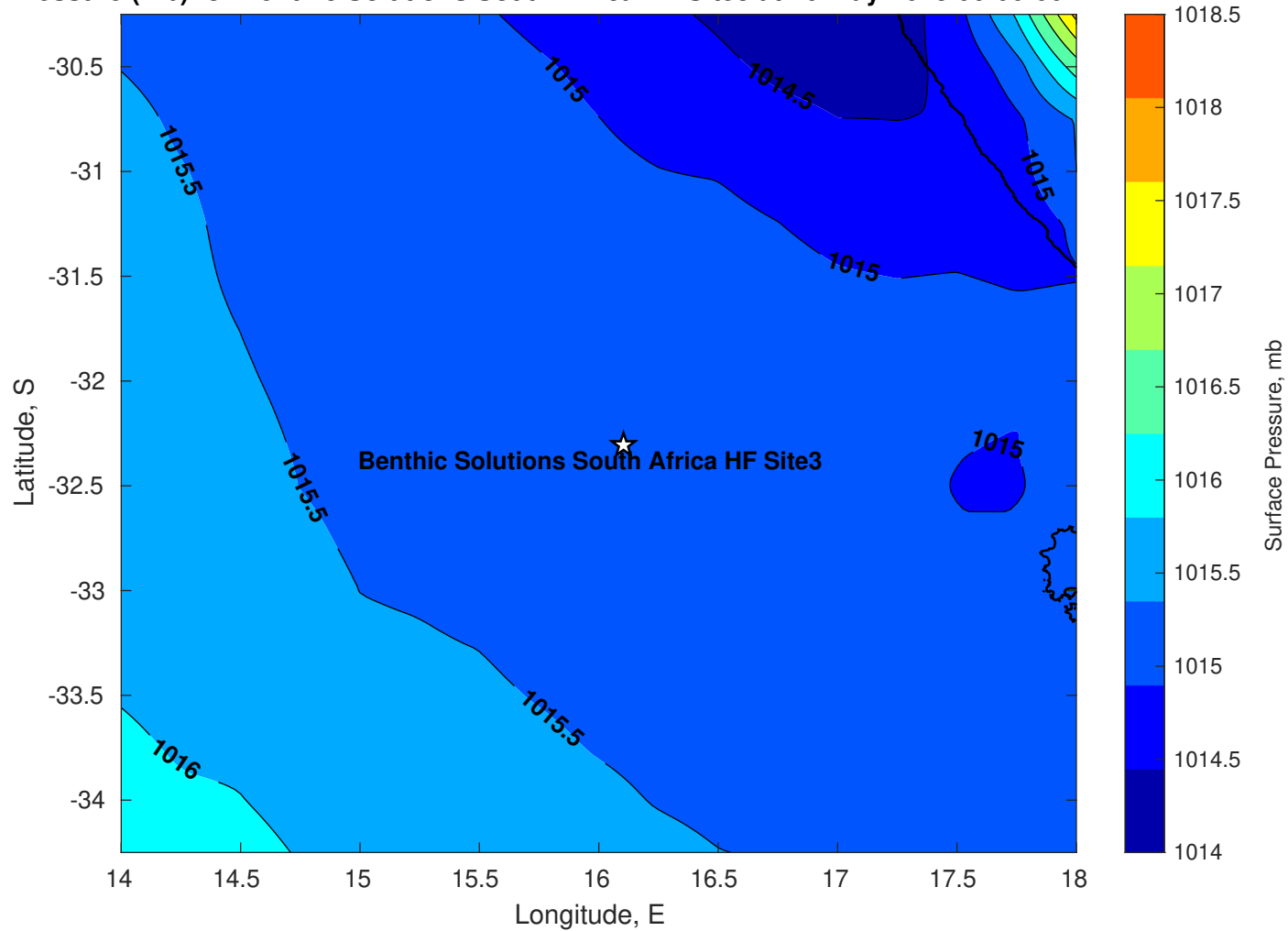
Surface Pressure (mb) for Benthic Solutions South Africa HF Site3 at 16-May-2025 00:00:00
