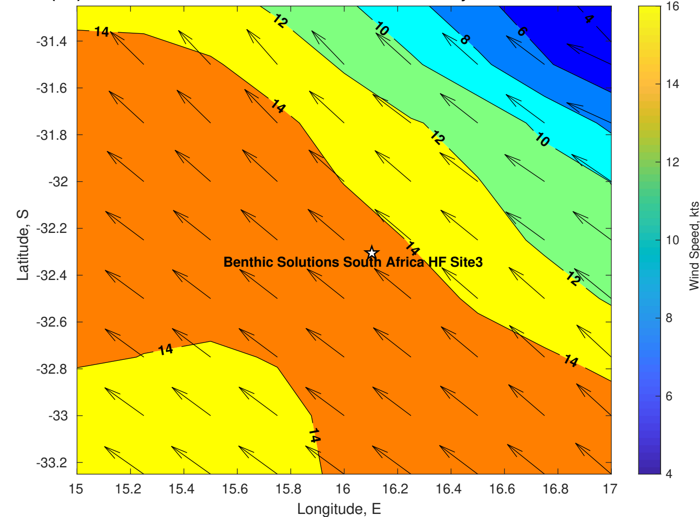
Winds (kts) for Benthic Solutions South Africa HF Site3 at 14-May-2025 09:00:00
