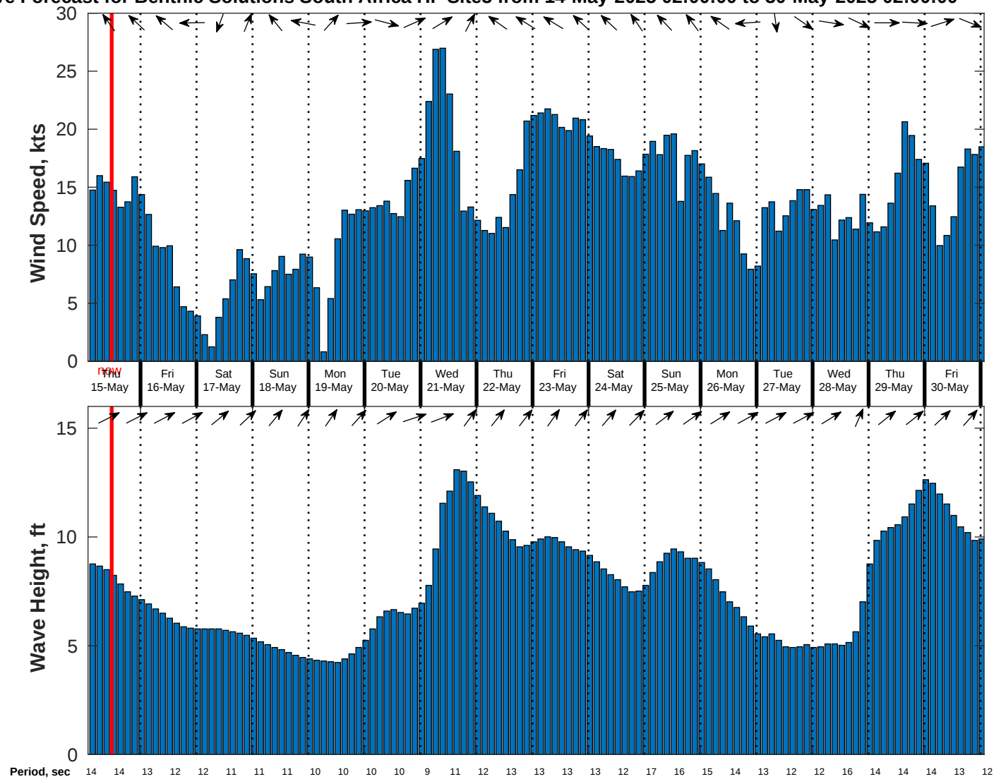
Wind & Wave Forecast for Benthic Solutions South Africa HF Site3 from 14-May-2025 02:00:00 to 30-May-2025 02:00:00
