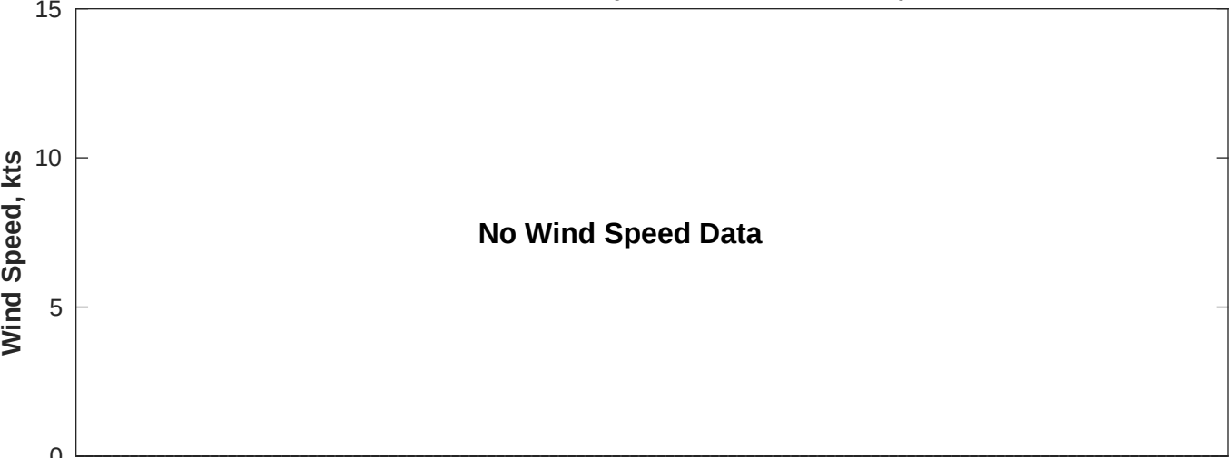
Wind & Wave Forecast for Brooks McCall from 13-May-2025 20:00:00 to 29-May-2025 20:00:00
