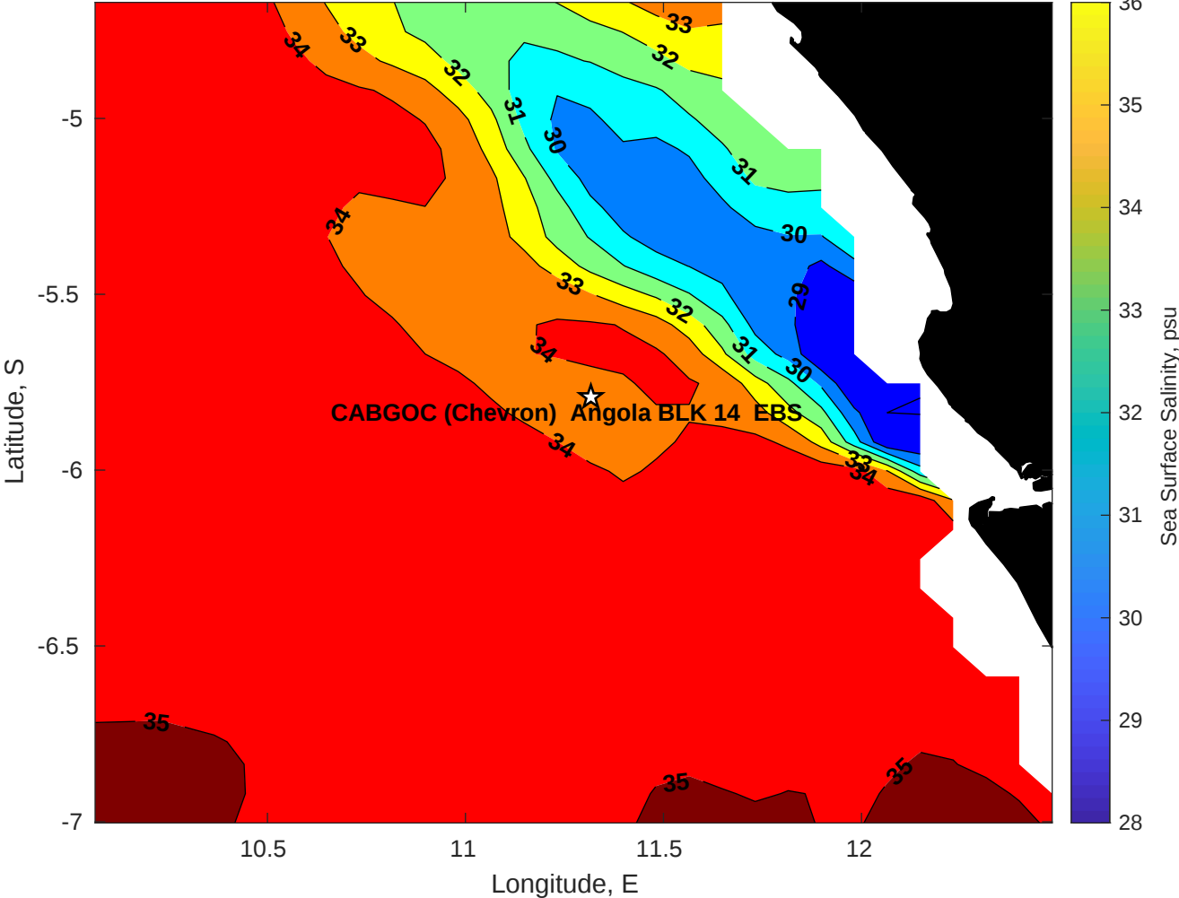
Surface Salinity for CABGOC (Chevron) Angola BLK 14 EBS at 13-May-2025 00:00:00
