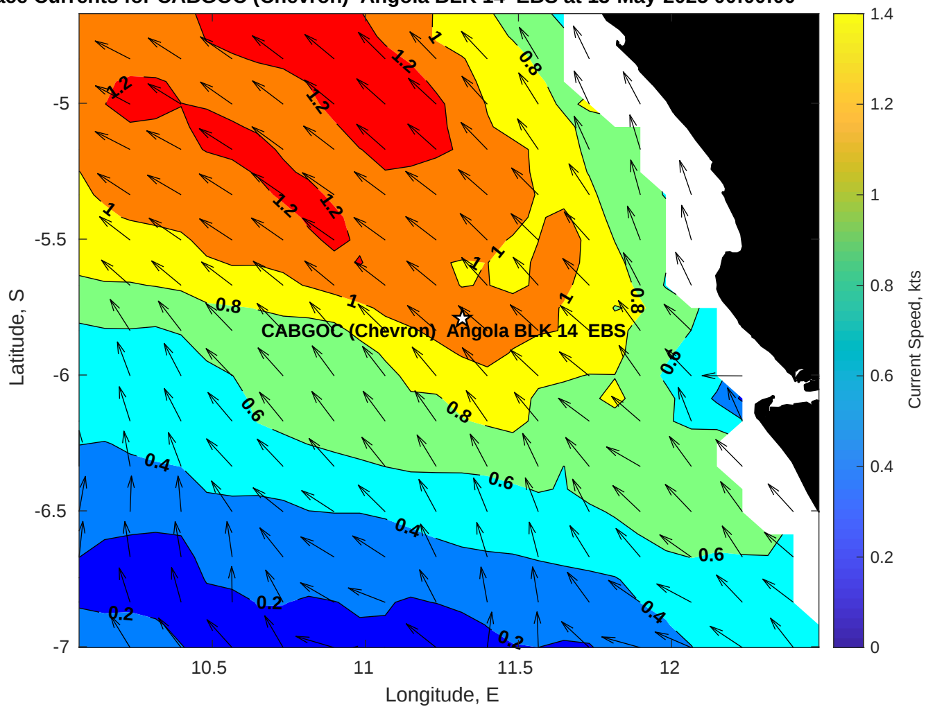
Surface Currents for CABGOC (Chevron) Angola BLK 14 EBS at 13-May-2025 00:00:00
