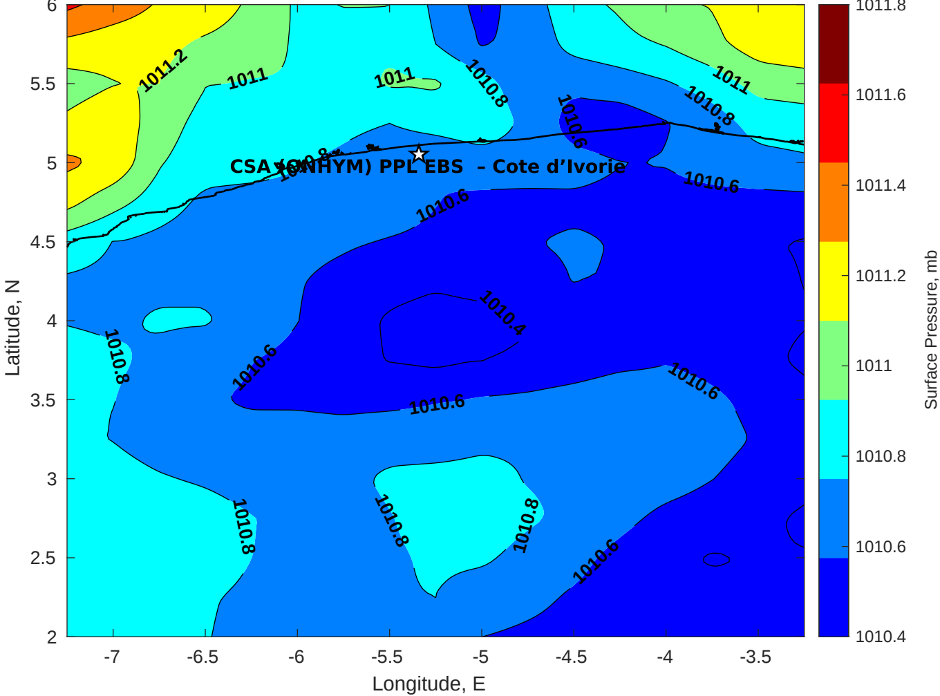
Surface Pressure (mb) for CSA (ONHYM) PPL EBS - Cote d'Ivoire at 16-May-2025 00:00:00
