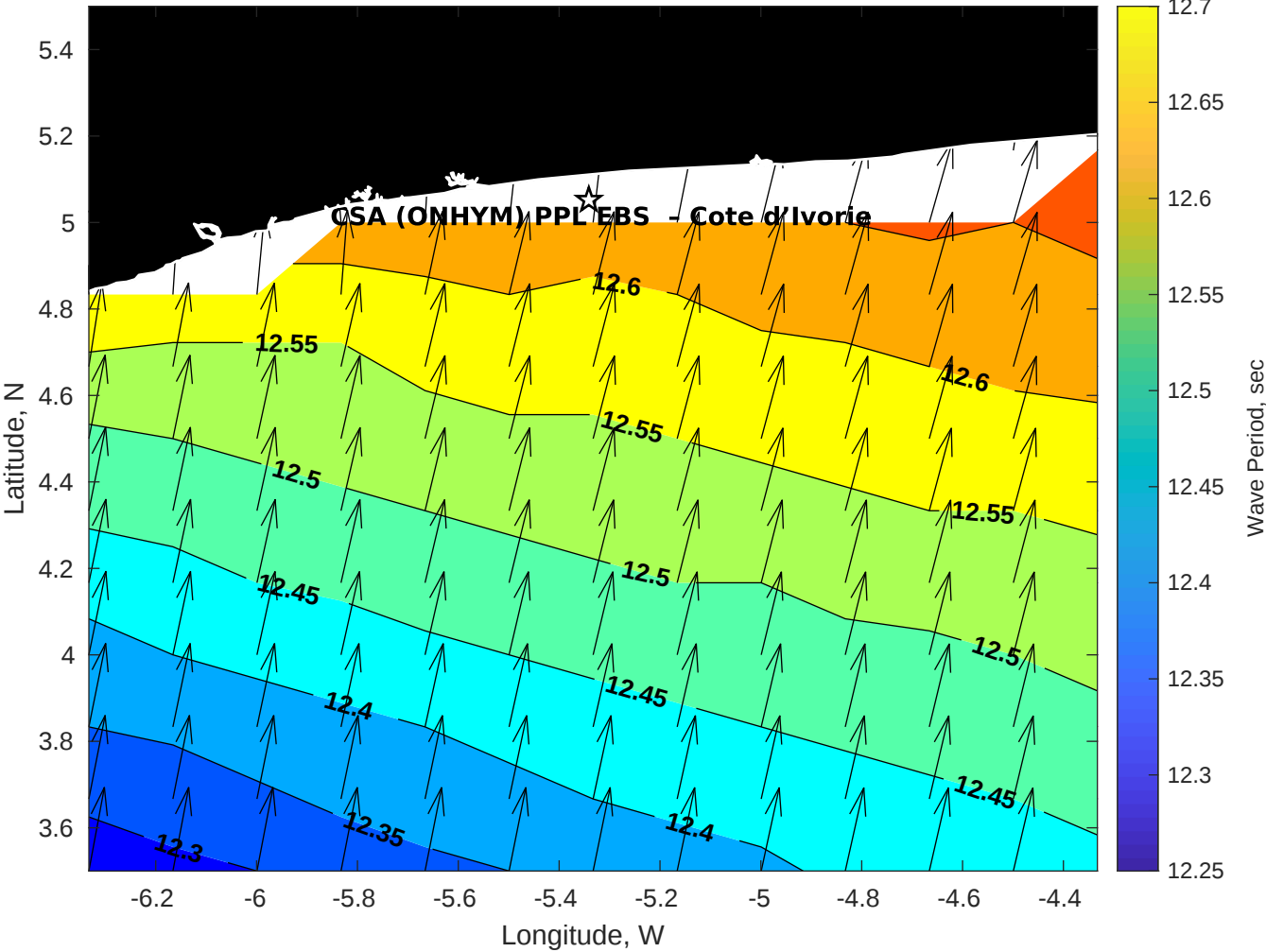
Wave Period (sec) for CSA (ONHYM) PPL EBS - Cote d'Ivoire at 14-May-2025 09:00:00
