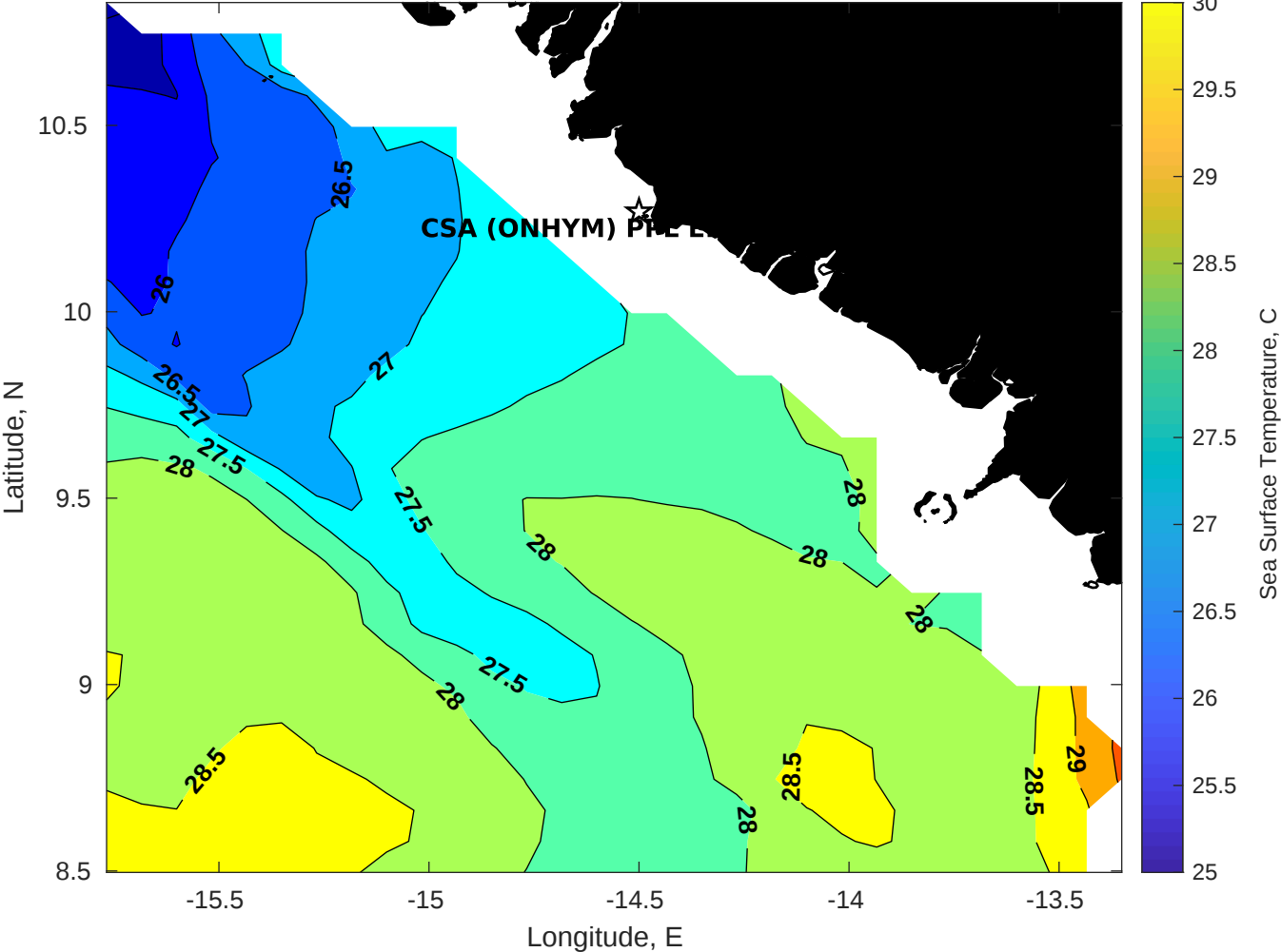
SST for CSA (ONHYM) PPL EBS - Guinea at 13-May-2025 00:00:00
