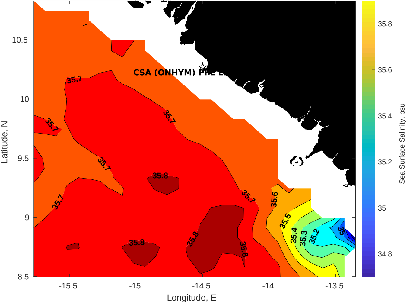
Surface Salinity for CSA (ONHYM) PPL EBS - Guinea at 13-May-2025 00:00:00
