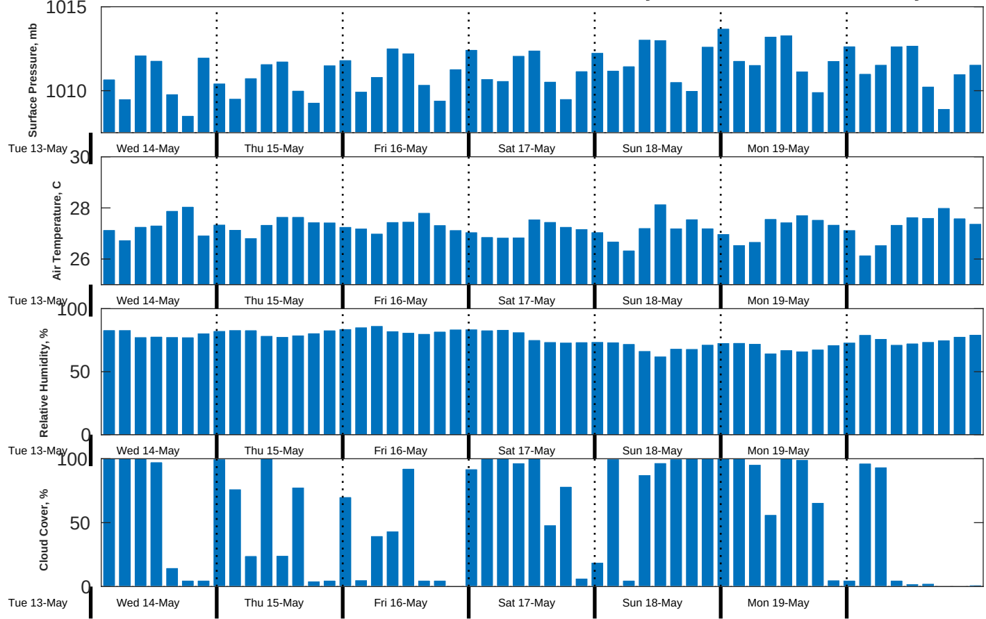
Met Forecast for CSA (ONHYM) PPL EBS - Guinea from 14-May-2025 00:00:00 to 21-May-2025 00:00:00
