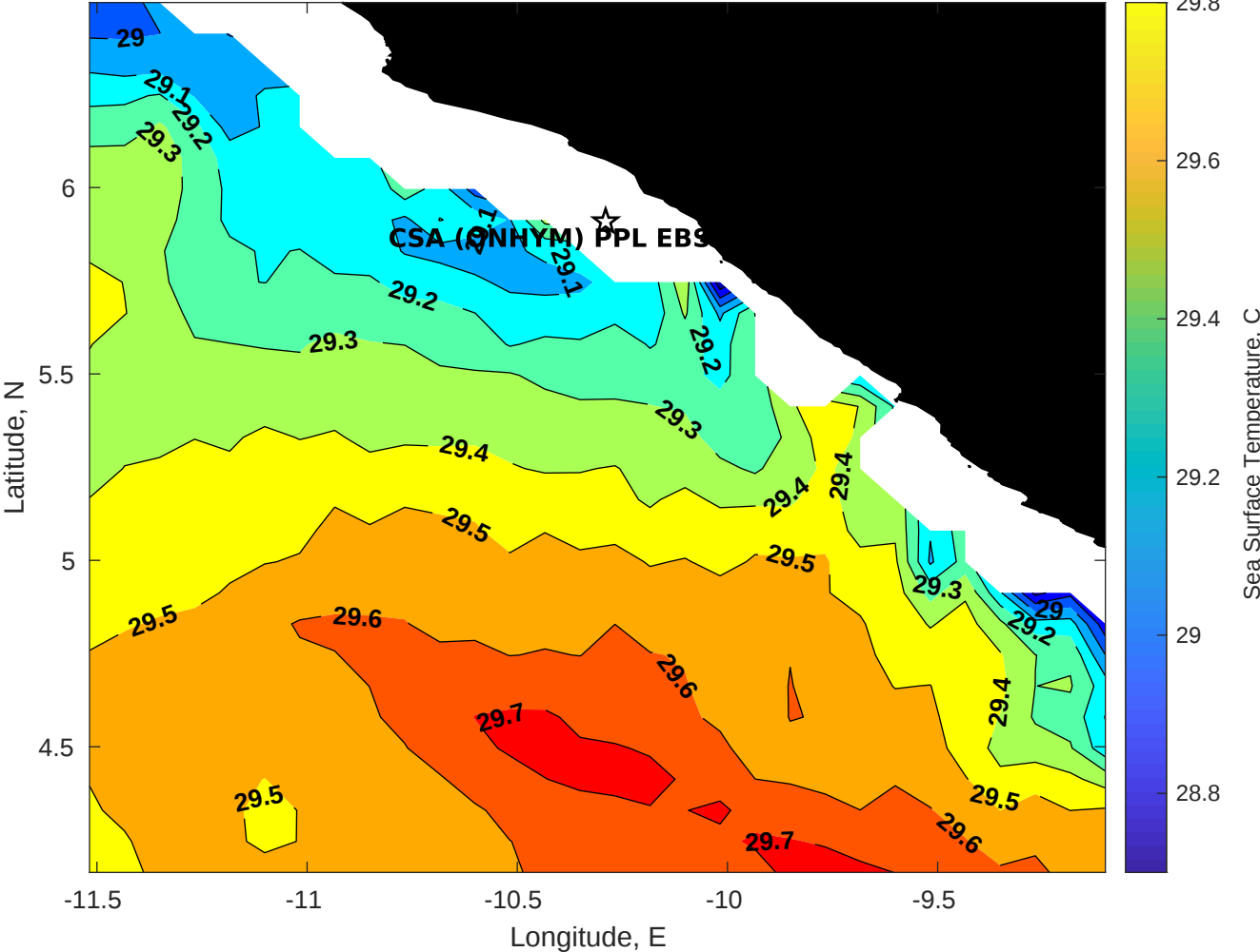
SST for CSA (ONHYM) PPL EBS - Liberia at 13-May-2025 00:00:00
