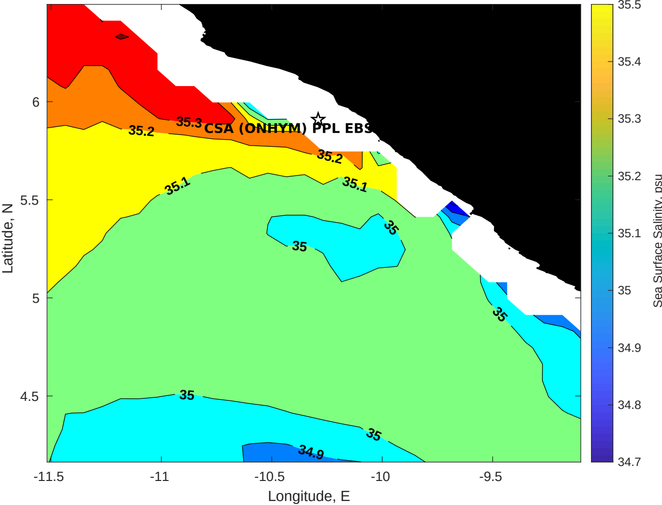
Surface Salinity for CSA (ONHYM) PPL EBS - Liberia at 13-May-2025 00:00:00
