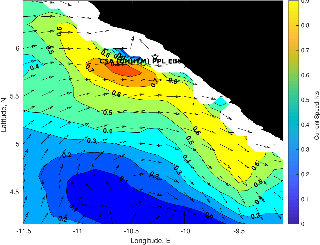
Surface Currents for CSA (ONHYM) PPL EBS - Liberia at 13-May-2025 00:00:00
