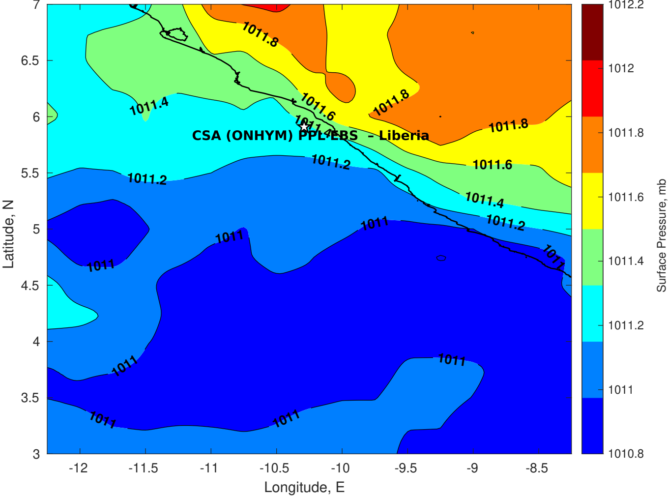
Surface Pressure (mb) for CSA (ONHYM) PPL EBS - Liberia at 16-May-2025 00:00:00
