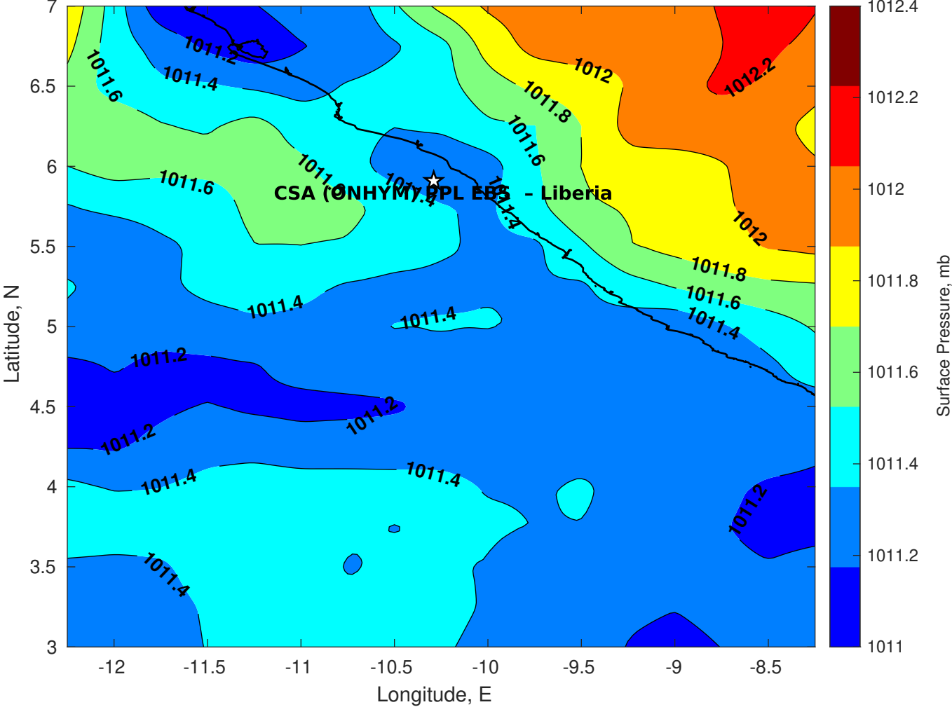
Surface Pressure (mb) for CSA (ONHYM) PPL EBS - Liberia at 15-May-2025 00:00:00
