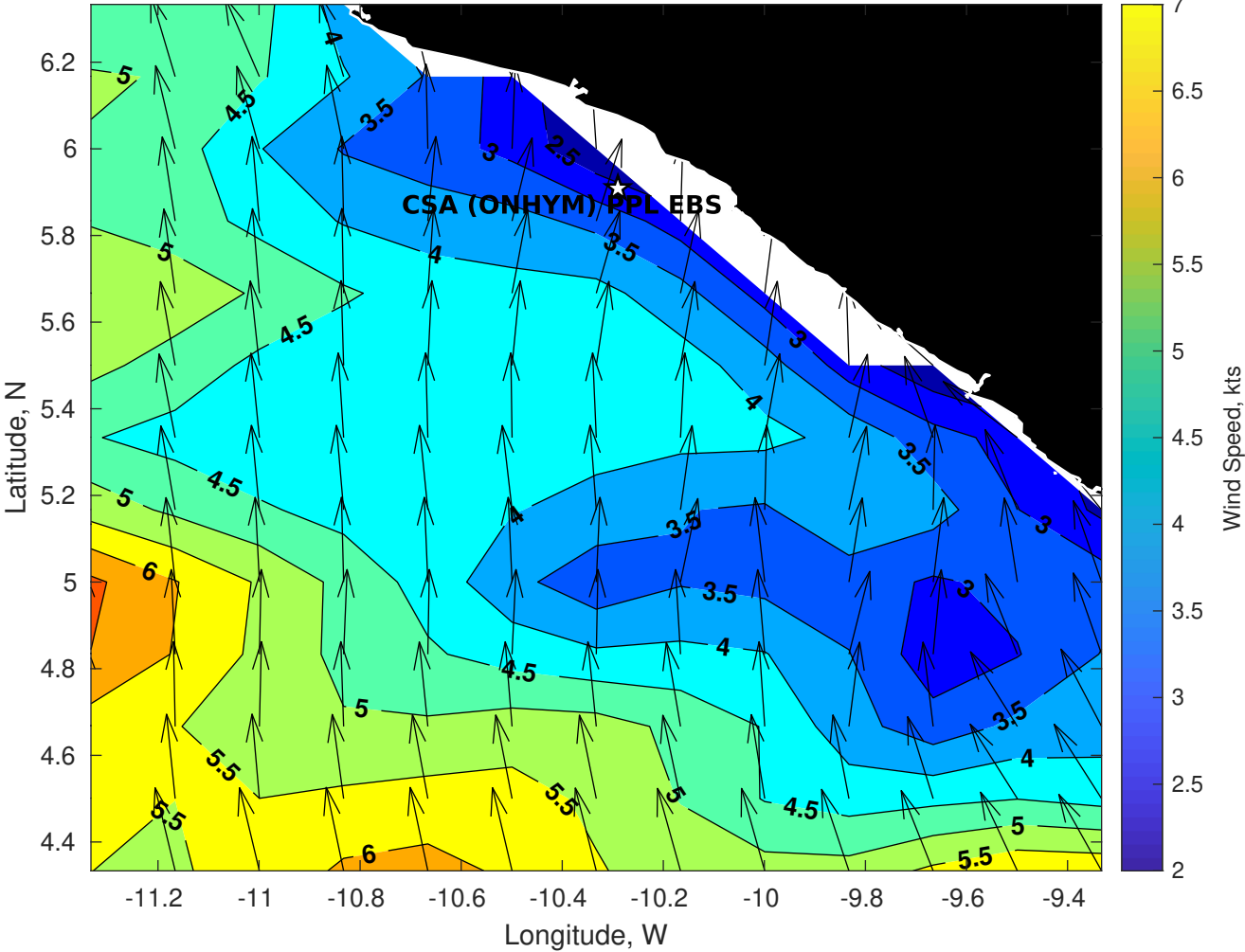
Winds (kts) for CSA (ONHYM) PPL EBS - Liberia at 14-May-2025 09:00:00
