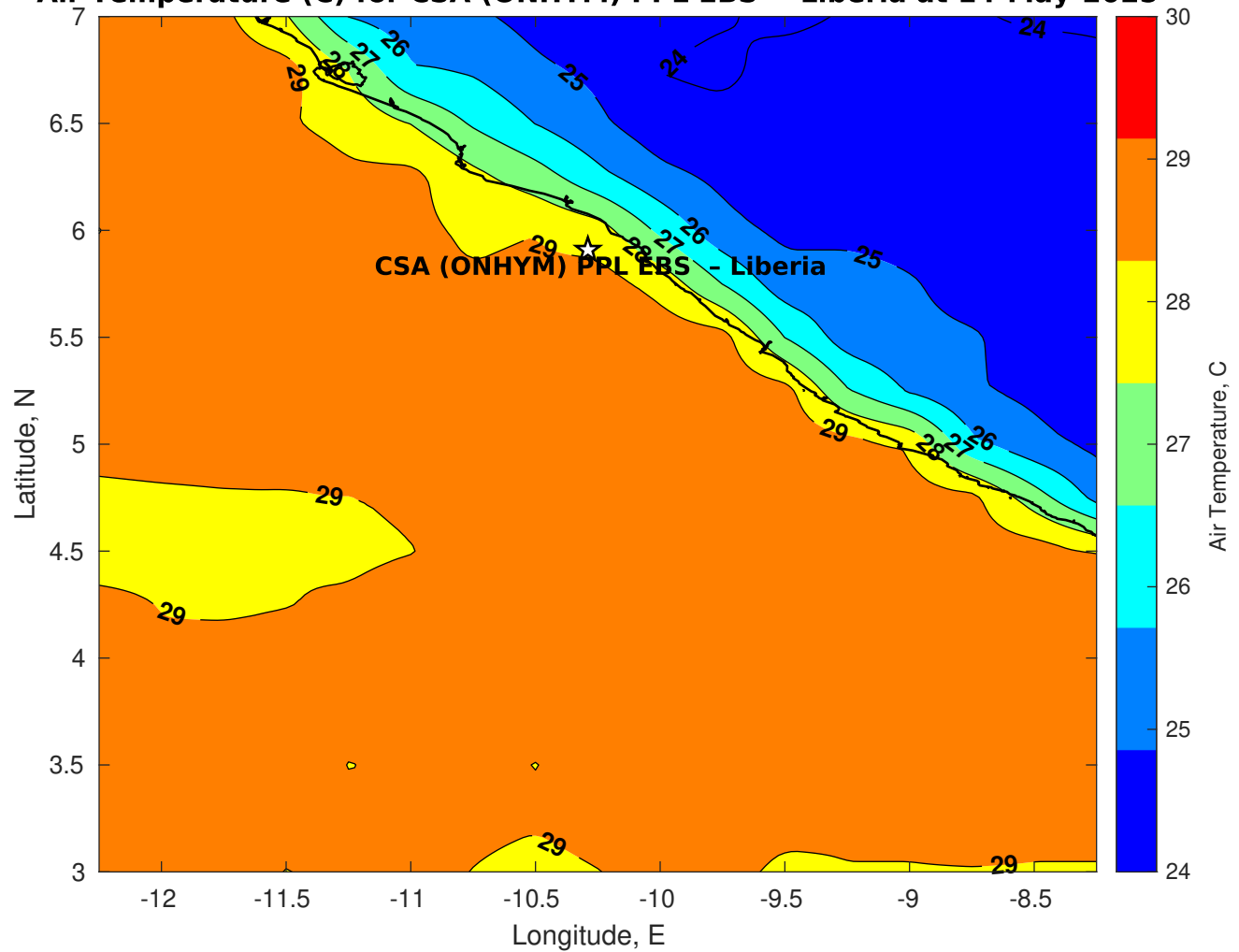
Air Temperature (C) for CSA (ONHYM) PPL EBS - Liberia at 14-May-2025
