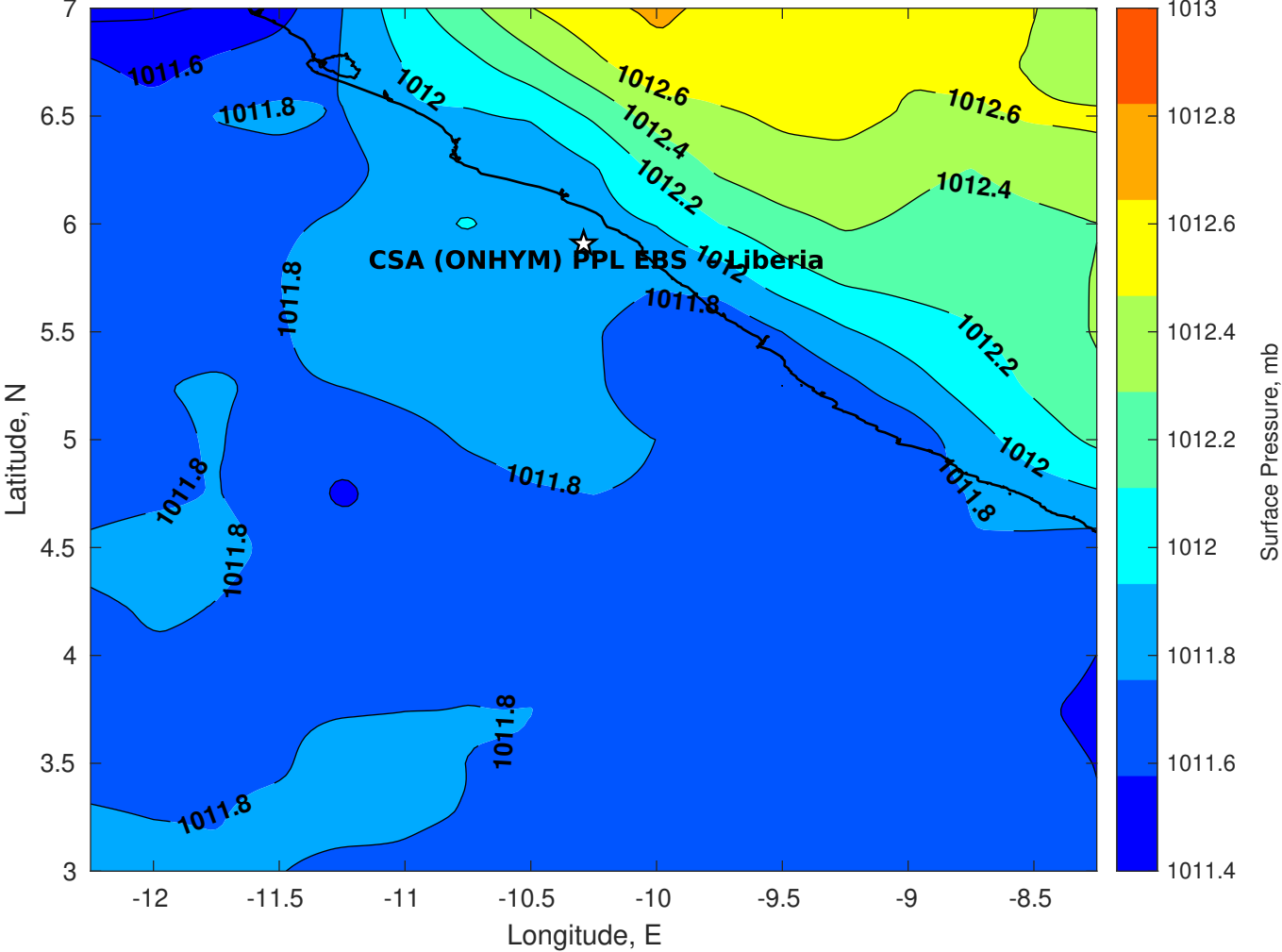
Surface Pressure (mb) for CSA (ONHYM) PPL EBS - Liberia at 14-May-2025 00:00:00
