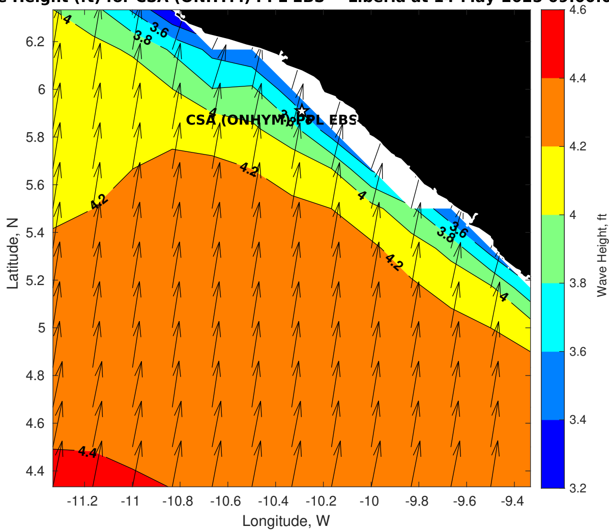
Wave Height (ft) for CSA (ONHYM) PPL EBS - Liberia at 14-May-2025 09:00:00
