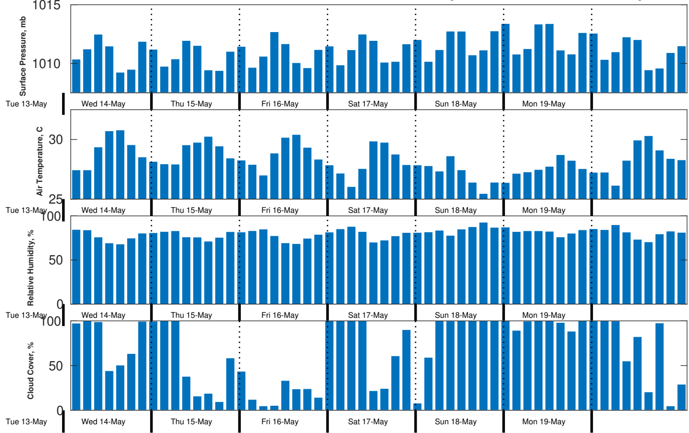
Met Forecast for CSA (ONHYM) PPL EBS - Liberia from 14-May-2025 00:00:00 to 21-May-2025 00:00:00
