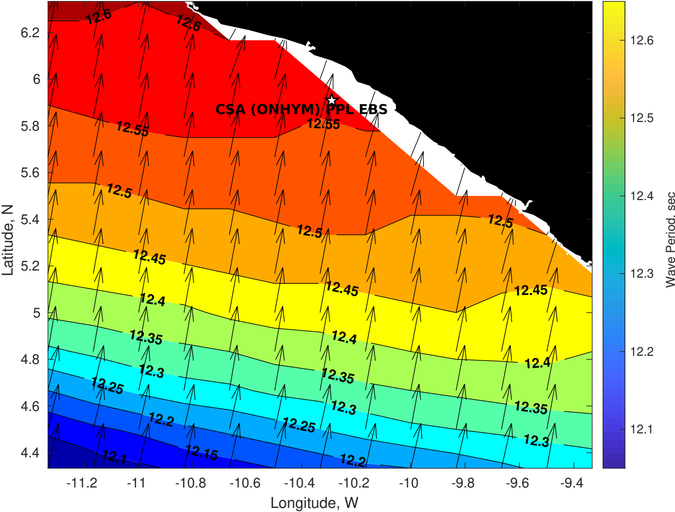
Wave Period (sec) for CSA (ONHYM) PPL EBS - Liberia at 14-May-2025 09:00:00
