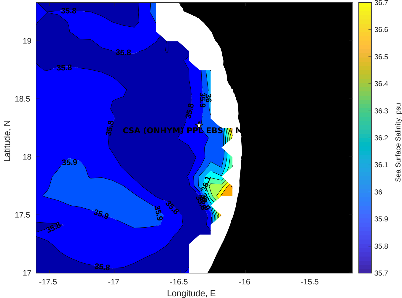
Surface Salinity for CSA (ONHYM) PPL EBS - Mauritania at 13-May-2025 00:00:00
