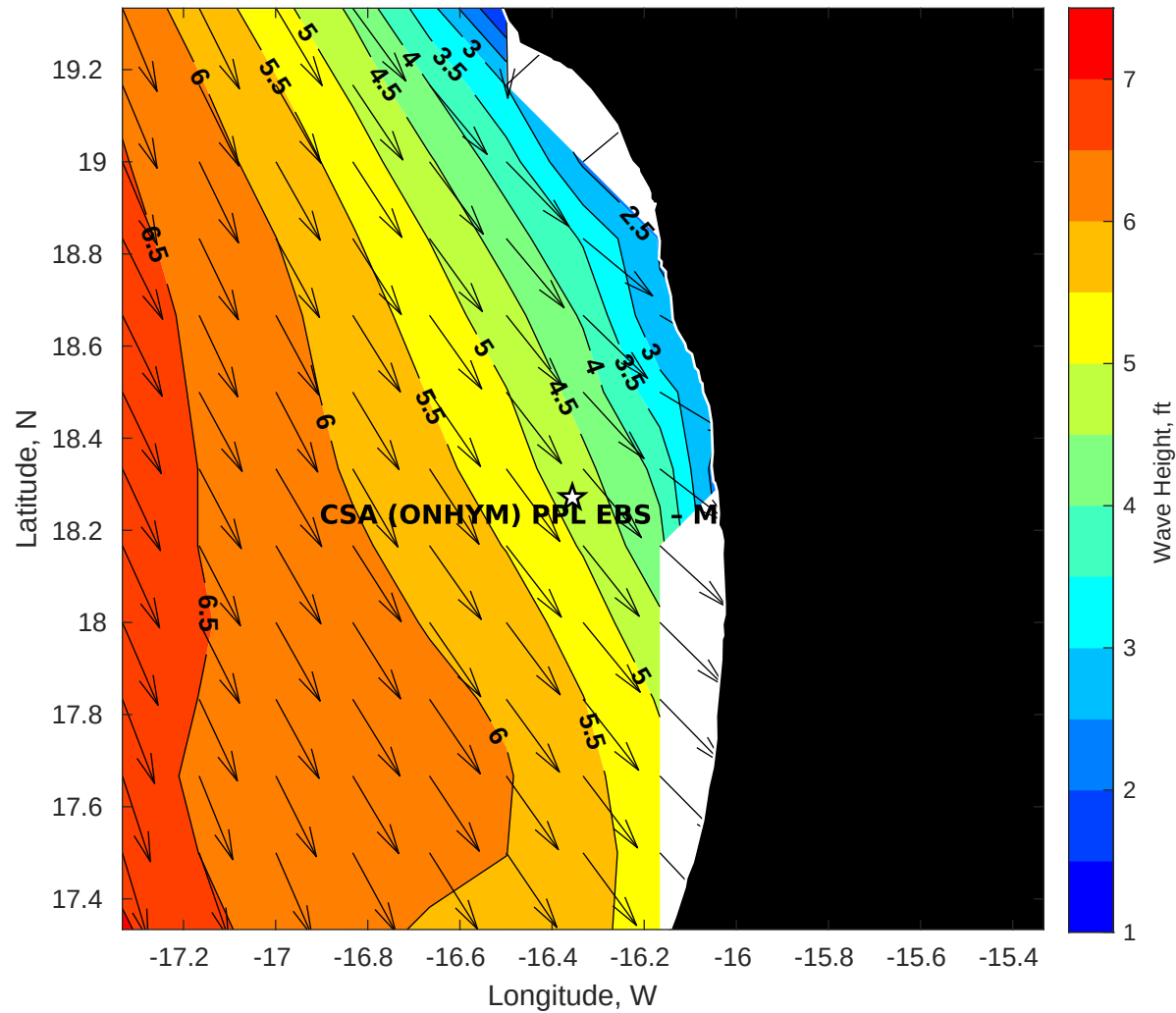
Wave Height (ft) for CSA (ONHYM) PPL EBS - Mauritania at 14-May-2025 09:00:00
