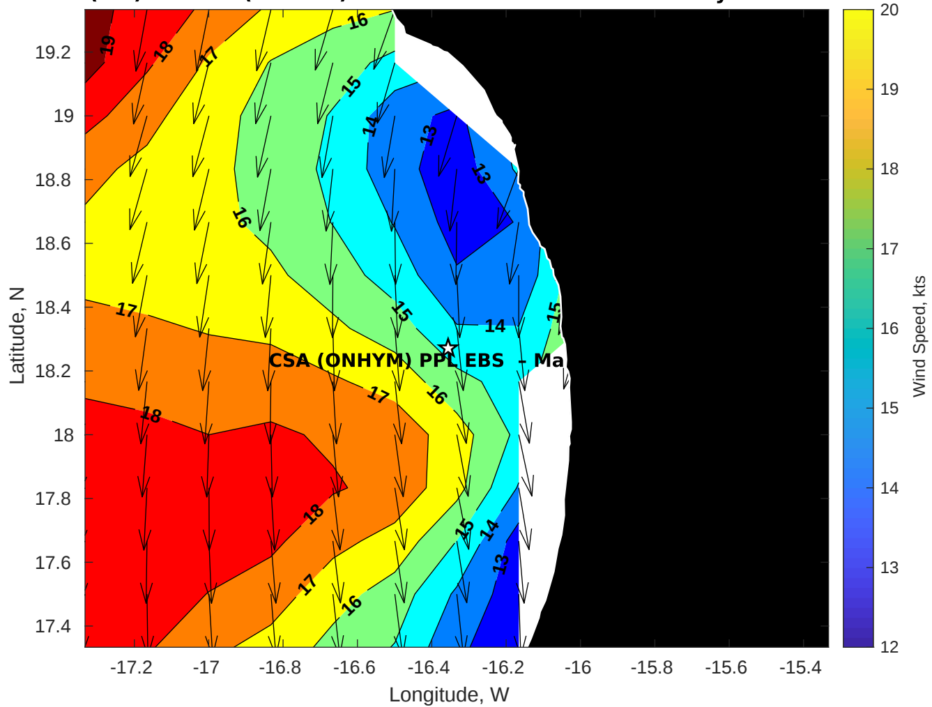
Winds (kts) for CSA (ONHYM) PPL EBS - Mauritania at 14-May-2025 09:00:00
