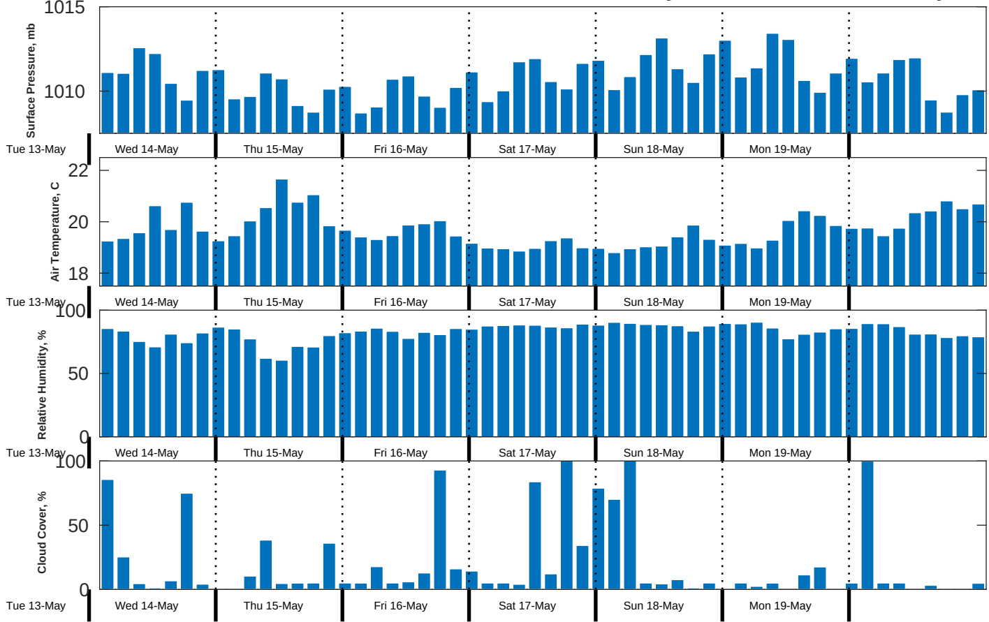
Met Forecast for CSA (ONHYM) PPL EBS - Mauritania from 14-May-2025 00:00:00 to 21-May-2025 00:00:00
