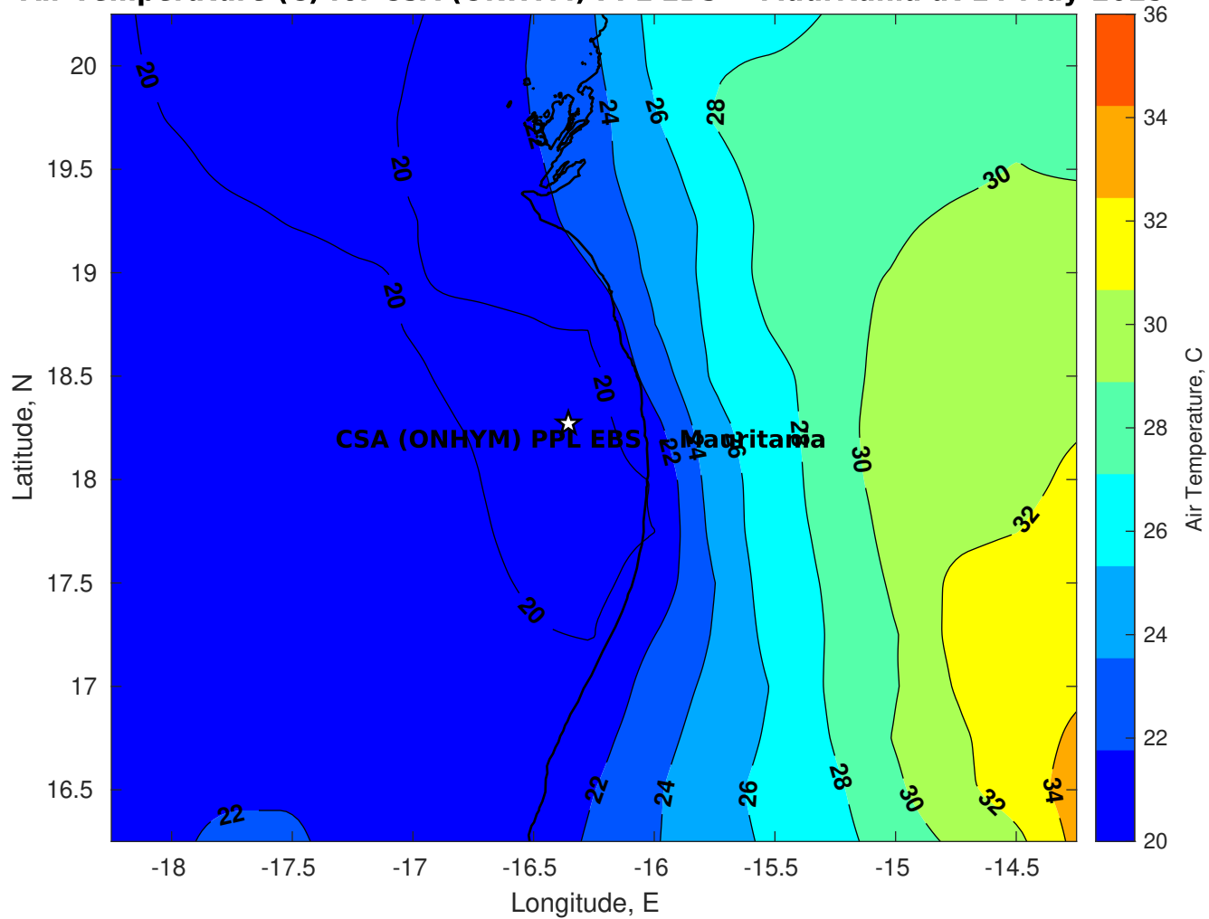
Air Temperature (C) for CSA (ONHYM) PPL EBS - Mauritania at 14-May-2025
