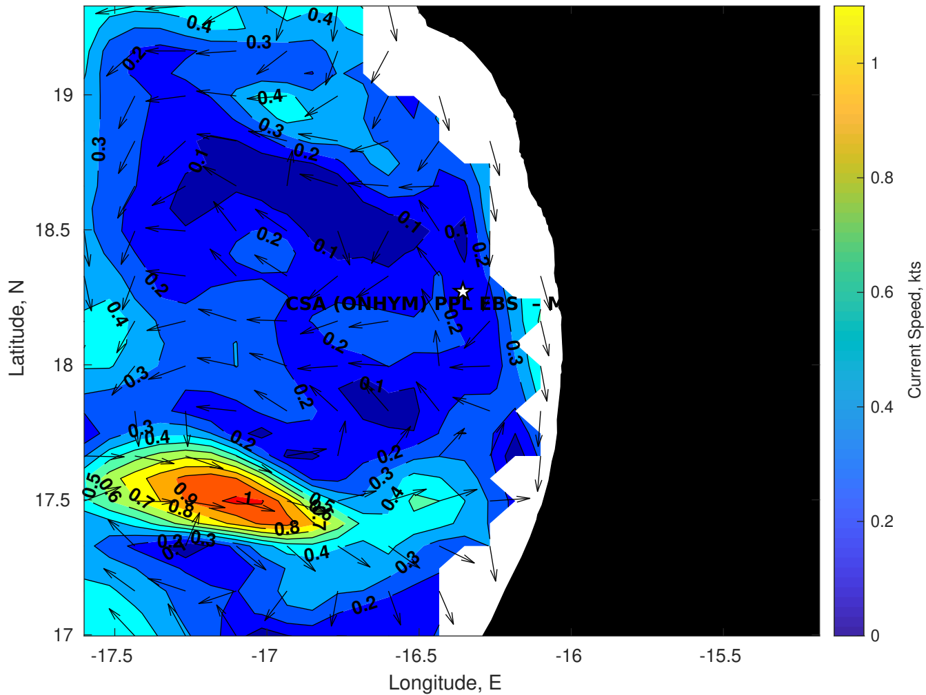
Surface Currents for CSA (ONHYM) PPL EBS - Mauritania at 13-May-2025 00:00:00
