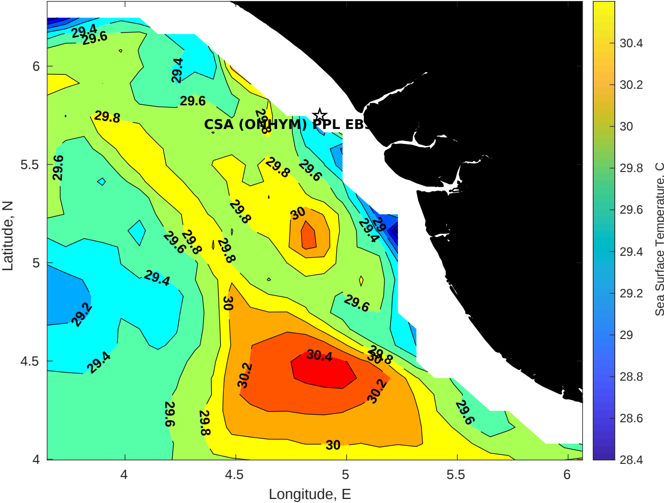
SST for CSA (ONHYM) PPL EBS - Nigeria at 13-May-2025 00:00:00
