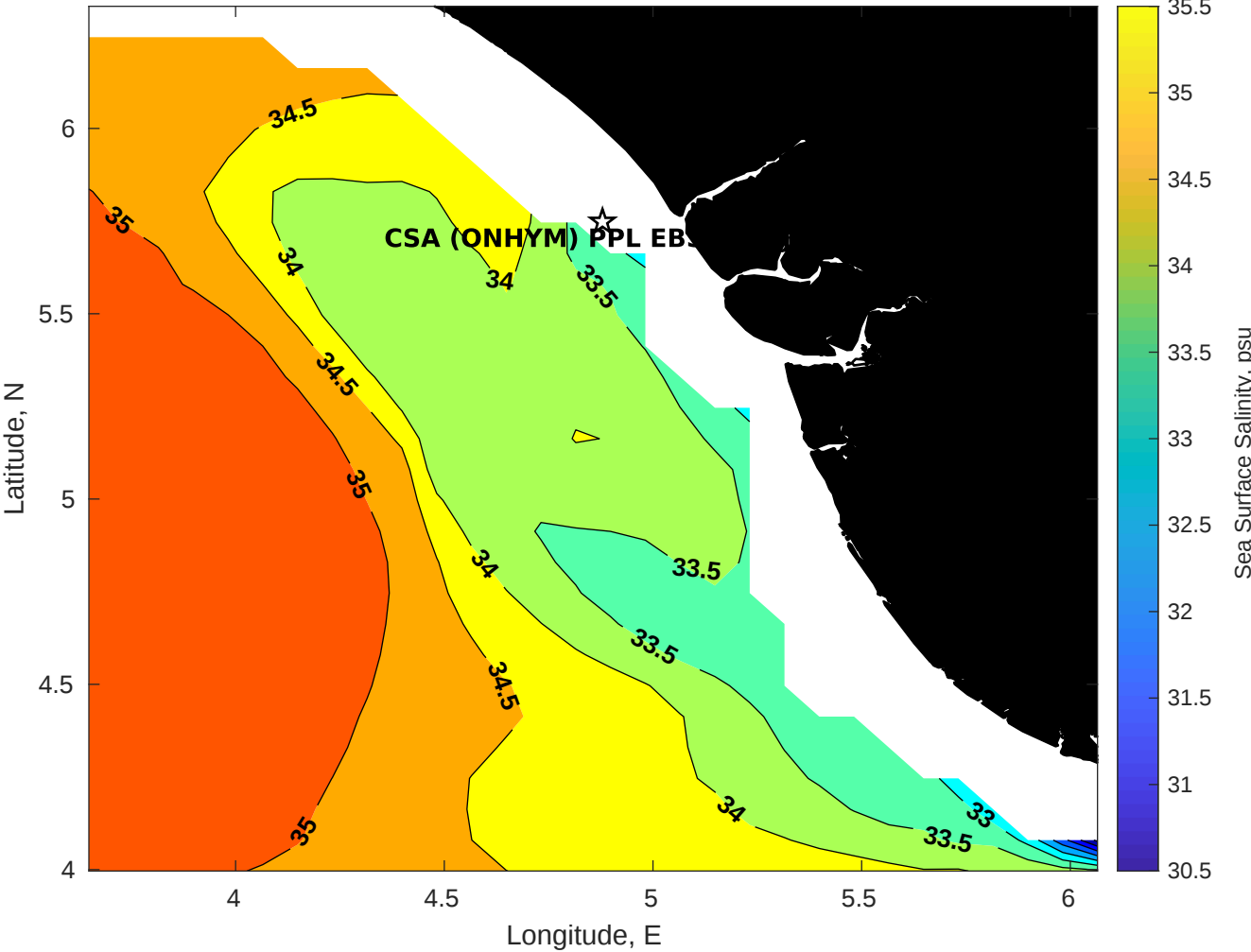
Surface Salinity for CSA (ONHYM) PPL EBS - Nigeria at 13-May-2025 00:00:00
