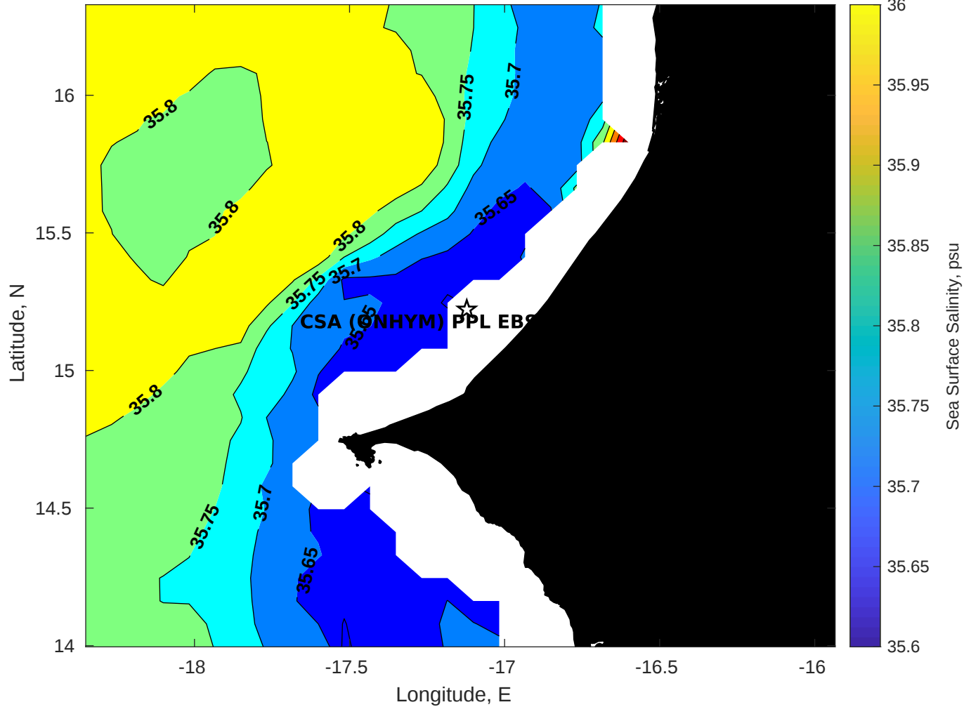
Surface Salinity for CSA (ONHYM) PPL EBS - Senegal at 13-May-2025 00:00:00
