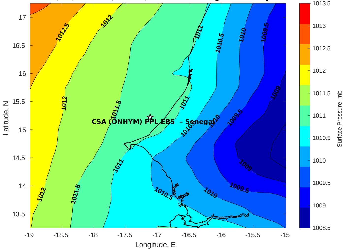
Surface Pressure (mb) for CSA (ONHYM) PPL EBS - Senegal at 15-May-2025 00:00:00
