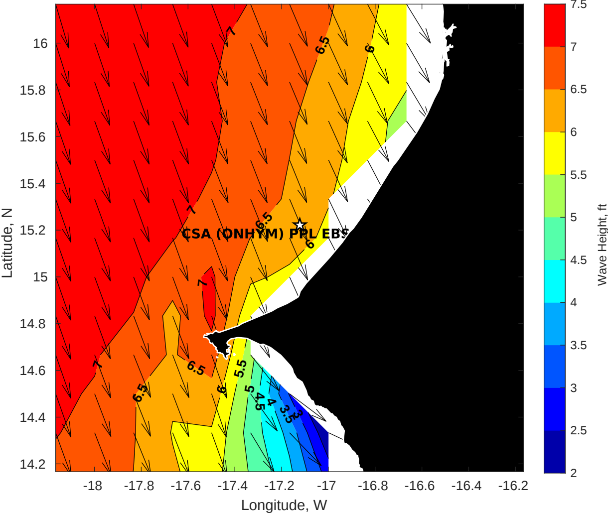
Wave Height (ft) for CSA (ONHYM) PPL EBS - Senegal at 14-May-2025 09:00:00
