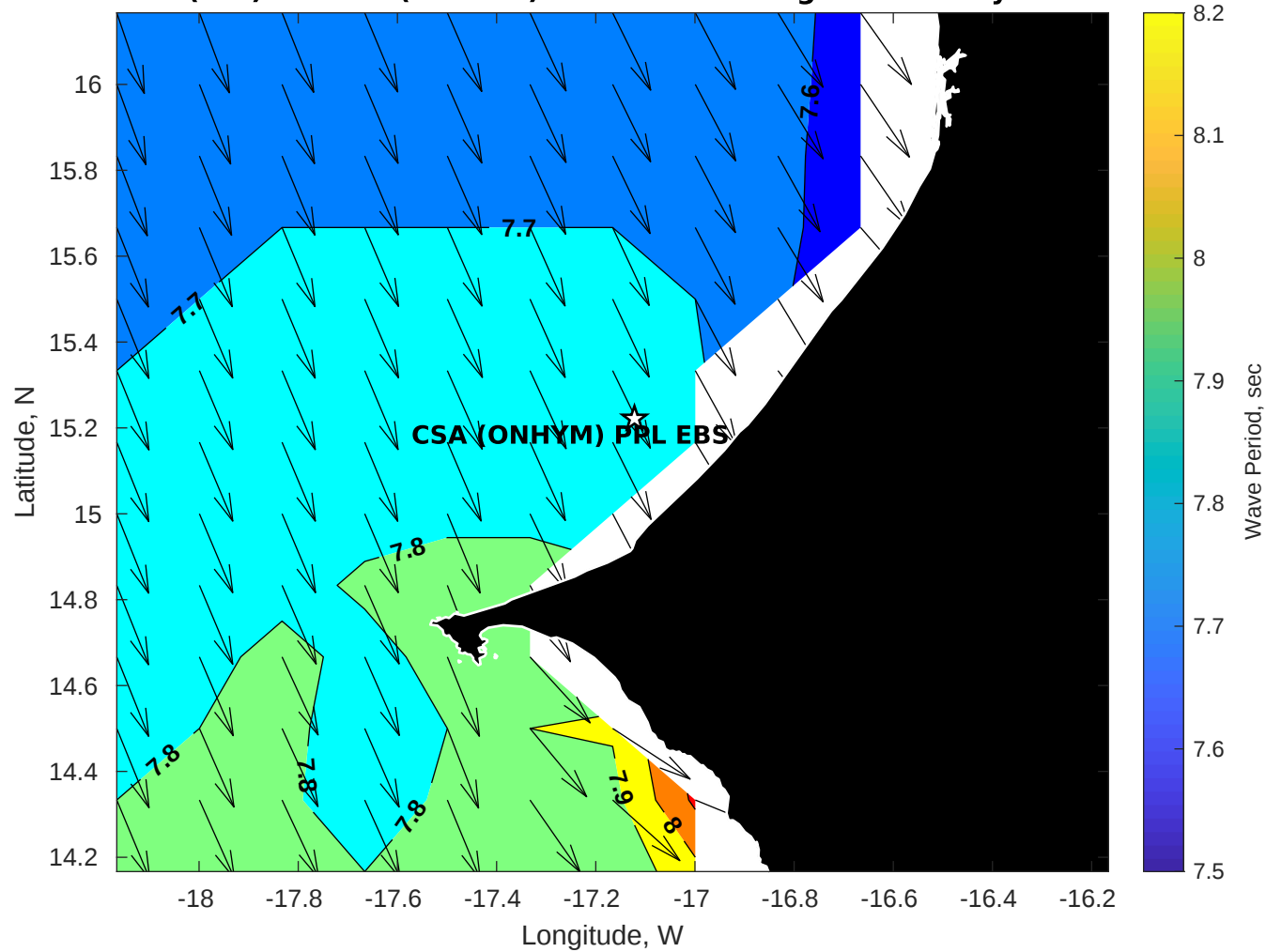
Wave Period (sec) for CSA (ONHYM) PPL EBS - Senegal at 14-May-2025 09:00:00
