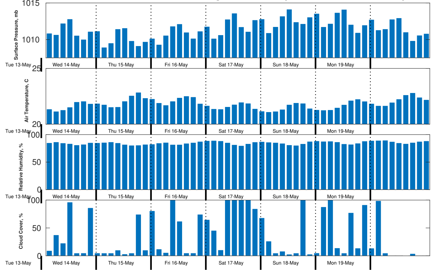
Met Forecast for CSA (ONHYM) PPL EBS - Senegal from 14-May-2025 00:00:00 to 21-May-2025 00:00:00
