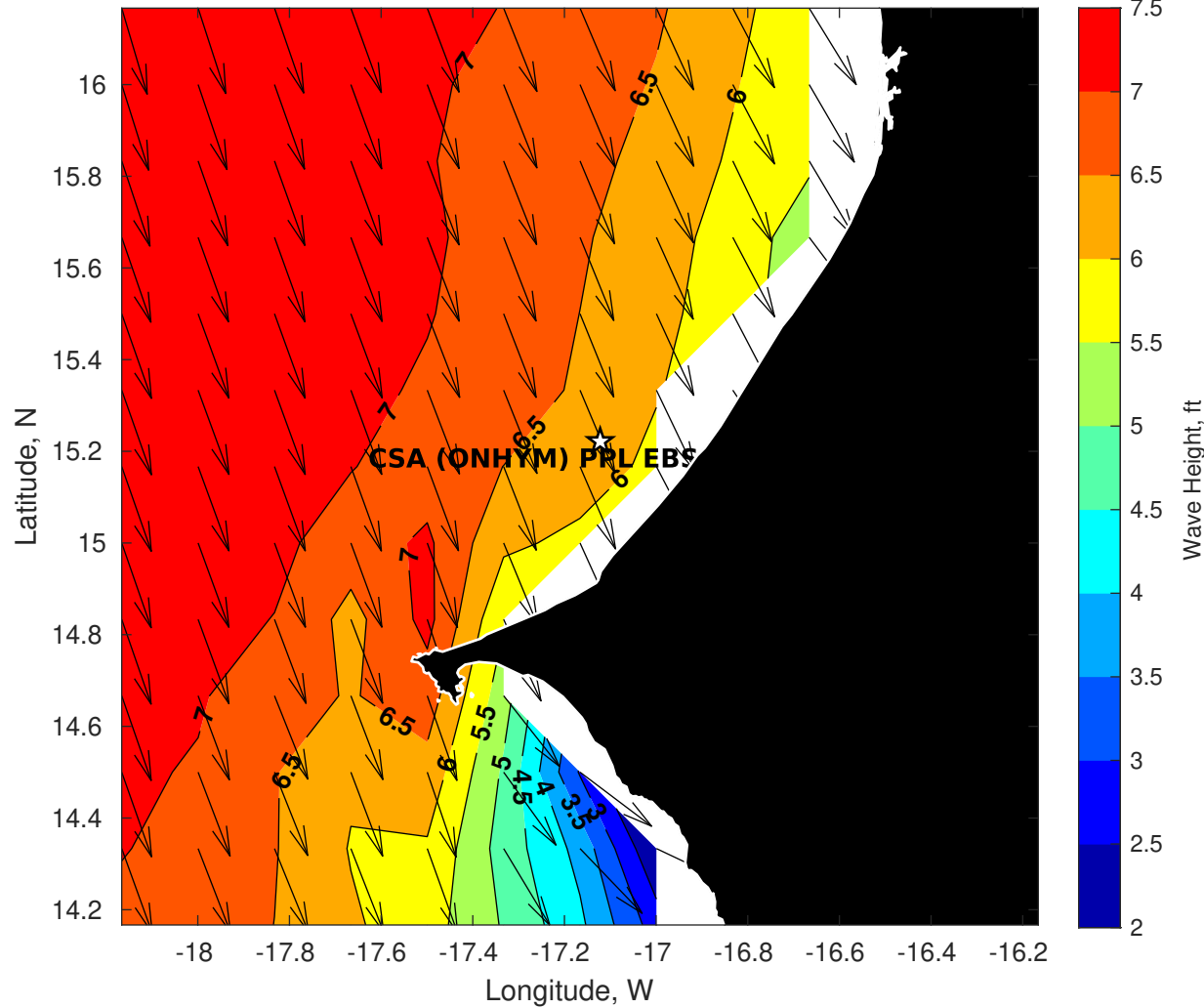
Wave Height (ft) for CSA (ONHYM) PPL EBS - Senegal at 14-May-2025 09:00:00
