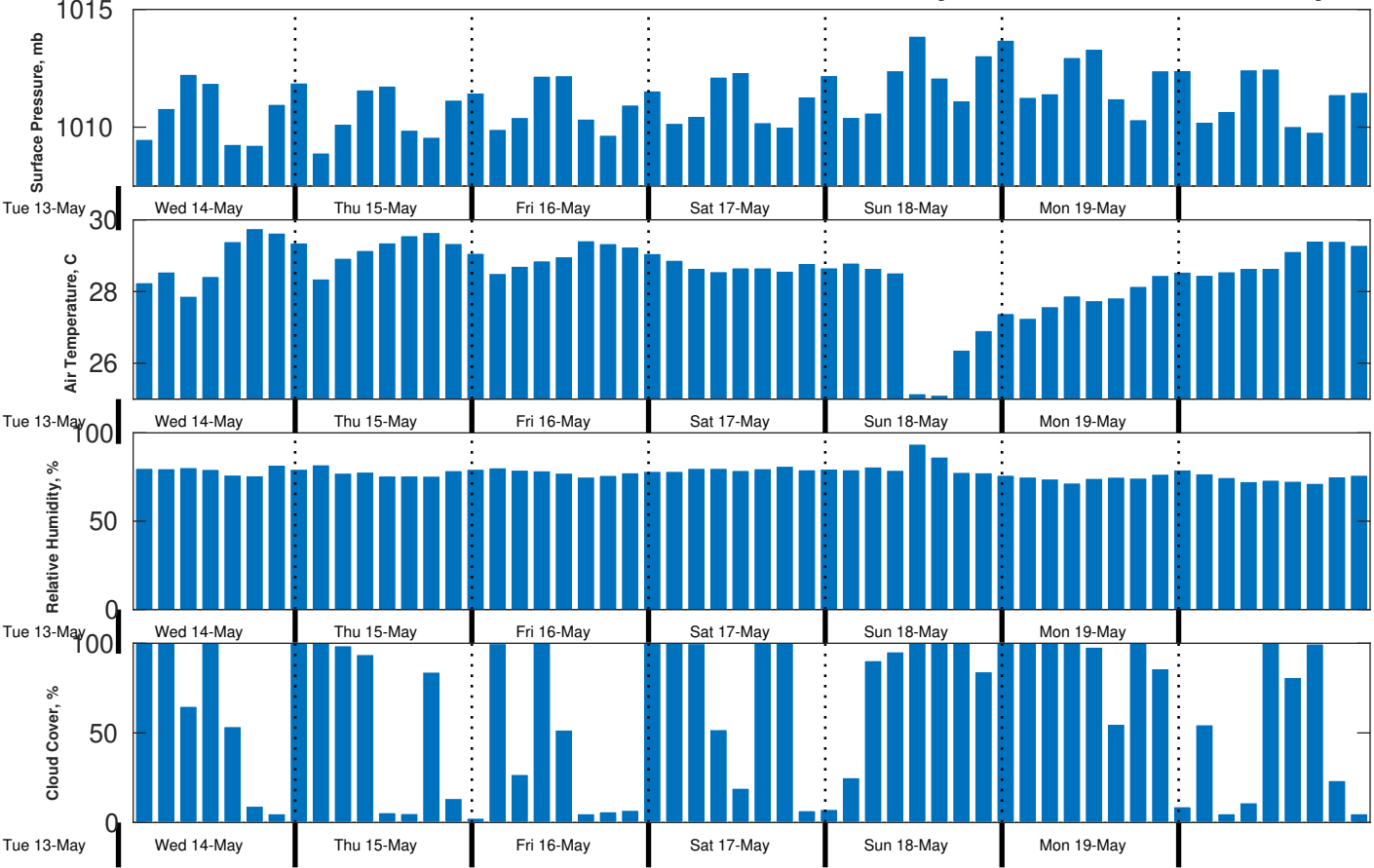
Met Forecast for CSA (ONHYM) PPL EBS - Sierra Leone from 14-May-2025 00:00:00 to 21-May-2025 00:00:00
