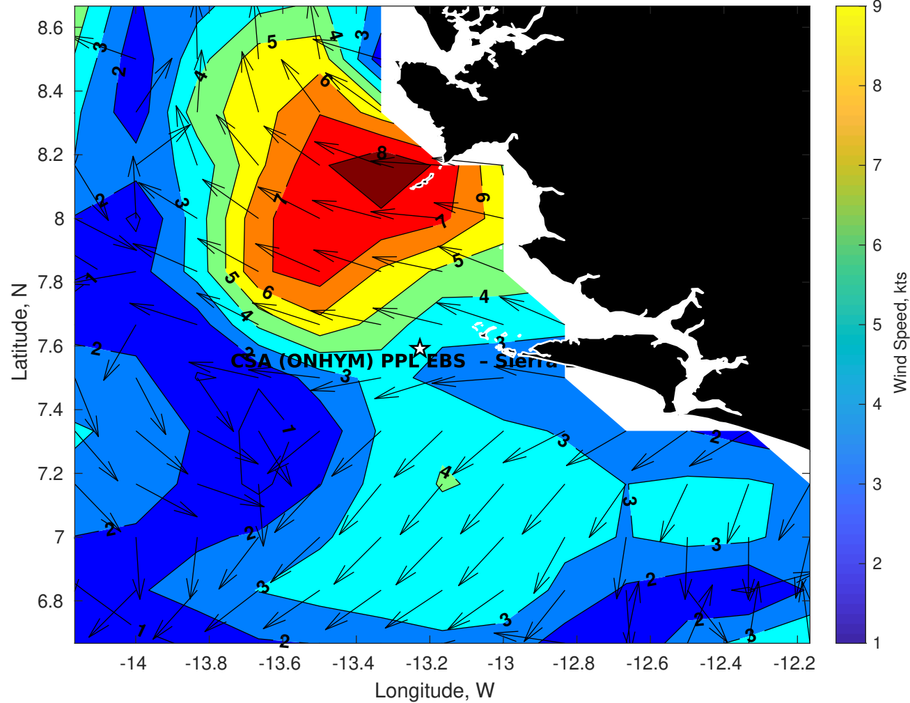
Winds (kts) for CSA (ONHYM) PPL EBS - Sierra Leone at 14-May-2025 09:00:00
