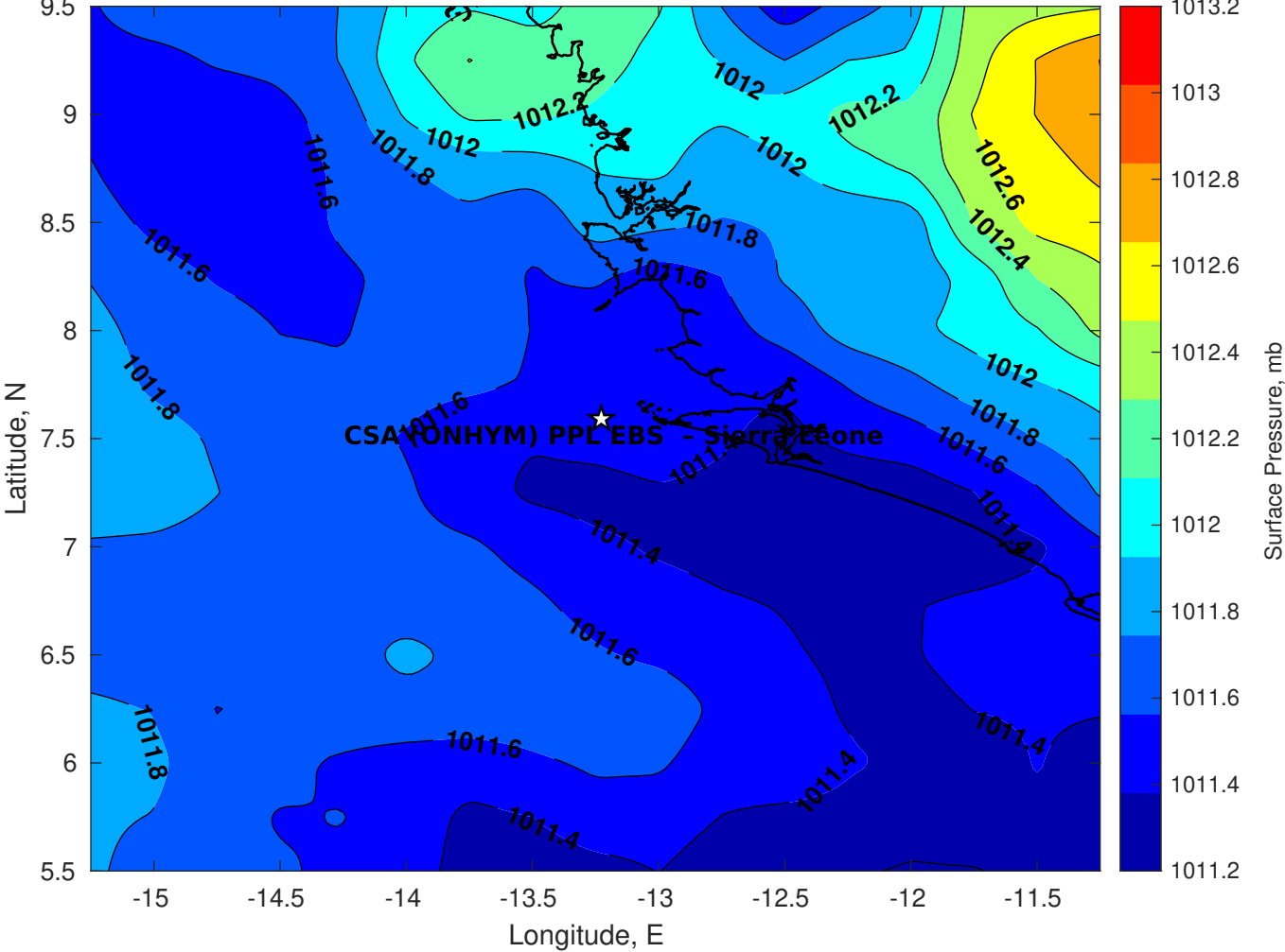
Surface Pressure (mb) for CSA (ONHYM) PPL EBS - Sierra Leone at 16-May-2025 00:00:00
