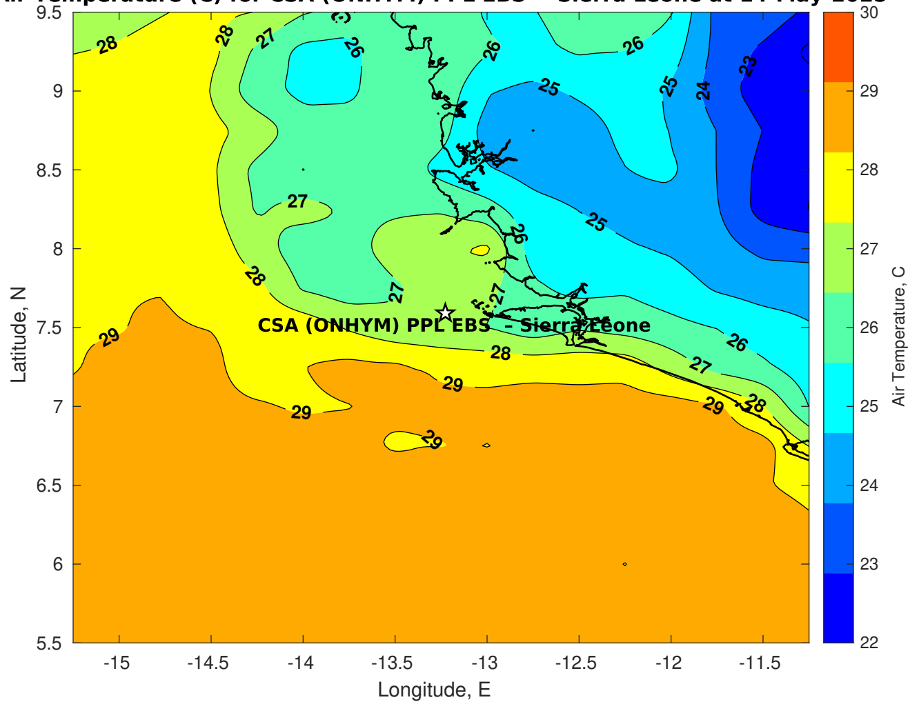
Air Temperature (C) for CSA (ONHYM) PPL EBS - Sierra Leone at 14-May-2025
