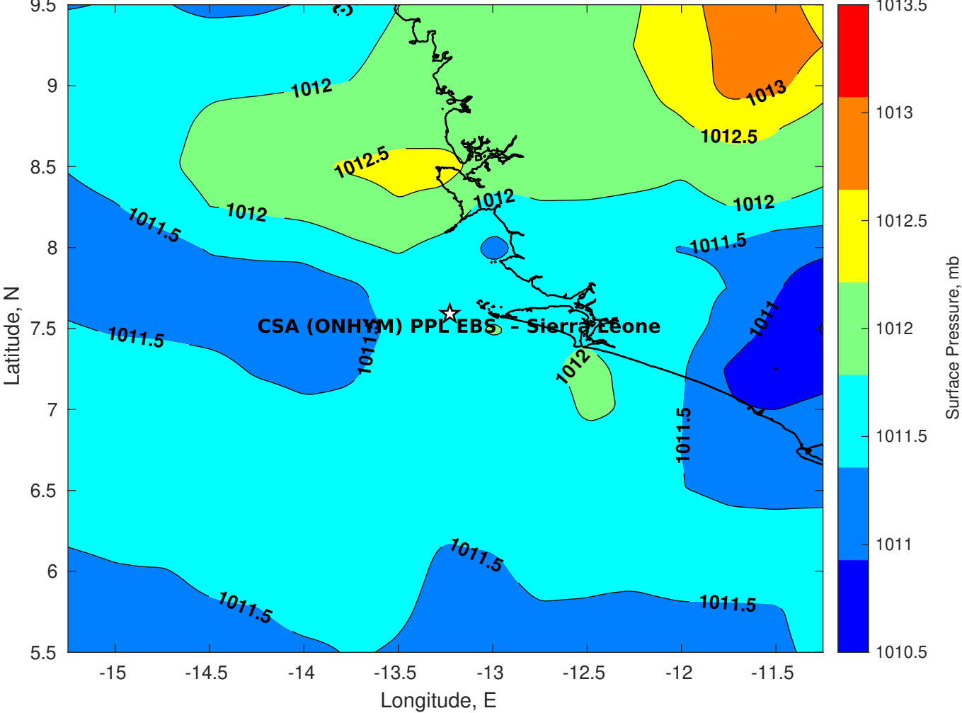
Surface Pressure (mb) for CSA (ONHYM) PPL EBS - Sierra Leone at 15-May-2025 00:00:00
