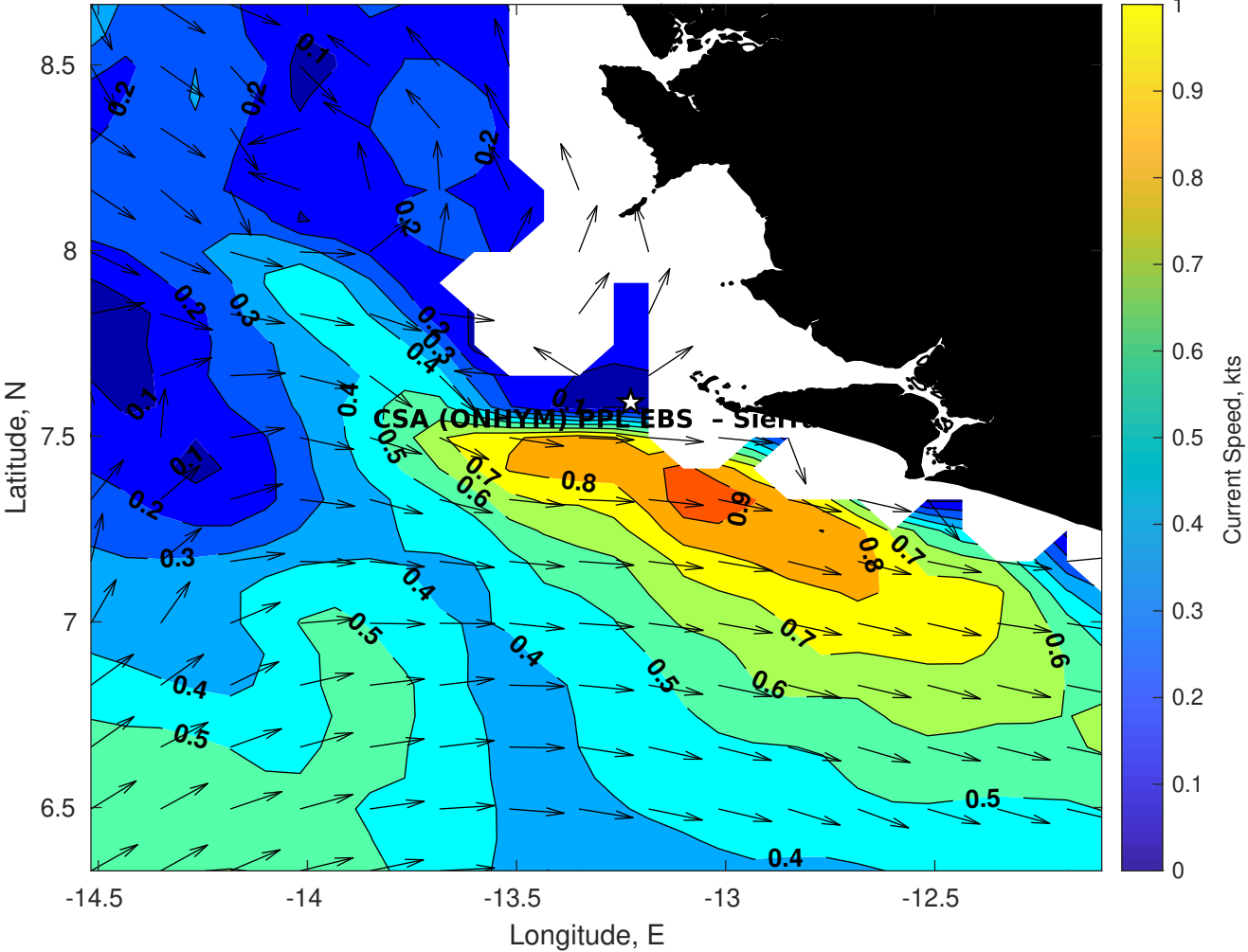
Surface Currents for CSA (ONHYM) PPL EBS - Sierra Leone at 13-May-2025 00:00:00
