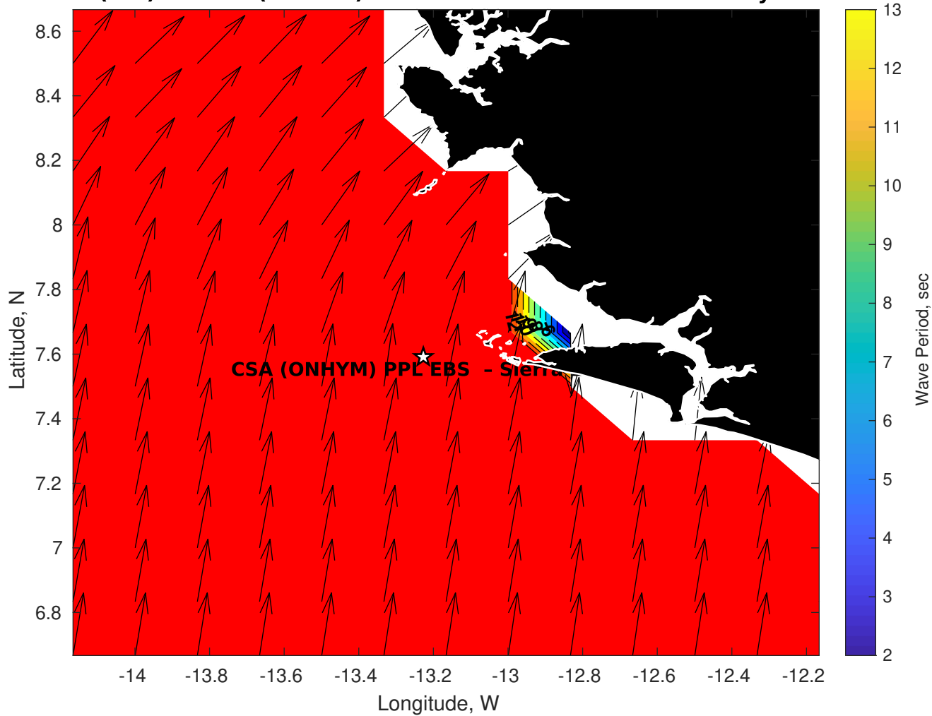
Wave Period (sec) for CSA (ONHYM) PPL EBS - Sierra Leone at 14-May-2025 09:00:00
