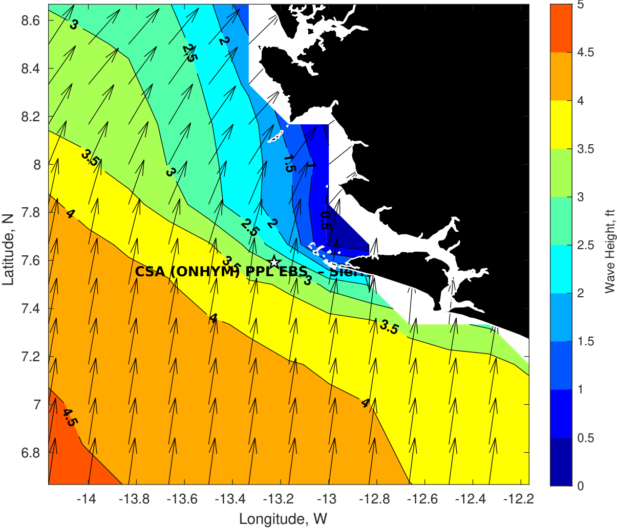
Wave Height (ft) for CSA (ONHYM) PPL EBS - Sierra Leone at 14-May-2025 09:00:00
