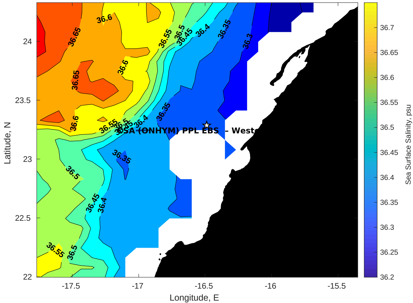
Surface Salinity for CSA (ONHYM) PPL EBS - Western Sahara at 13-May-2025 00:00:00
