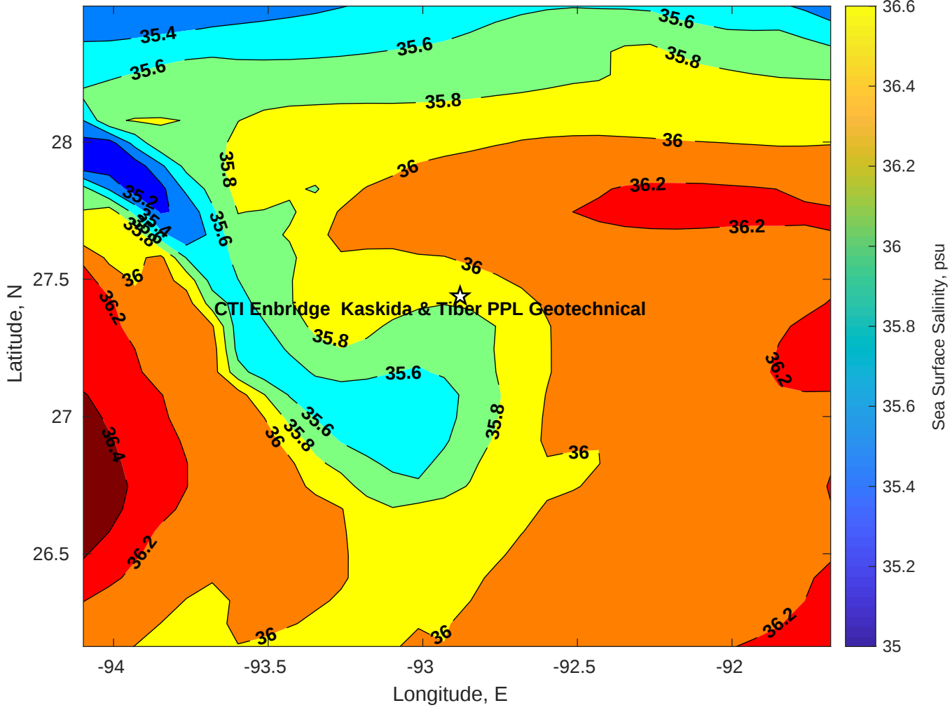
Surface Salinity for CTI Enbridge Kaskida & Tiber PPL Geotechnical at 13-May-2025 00:00:00
