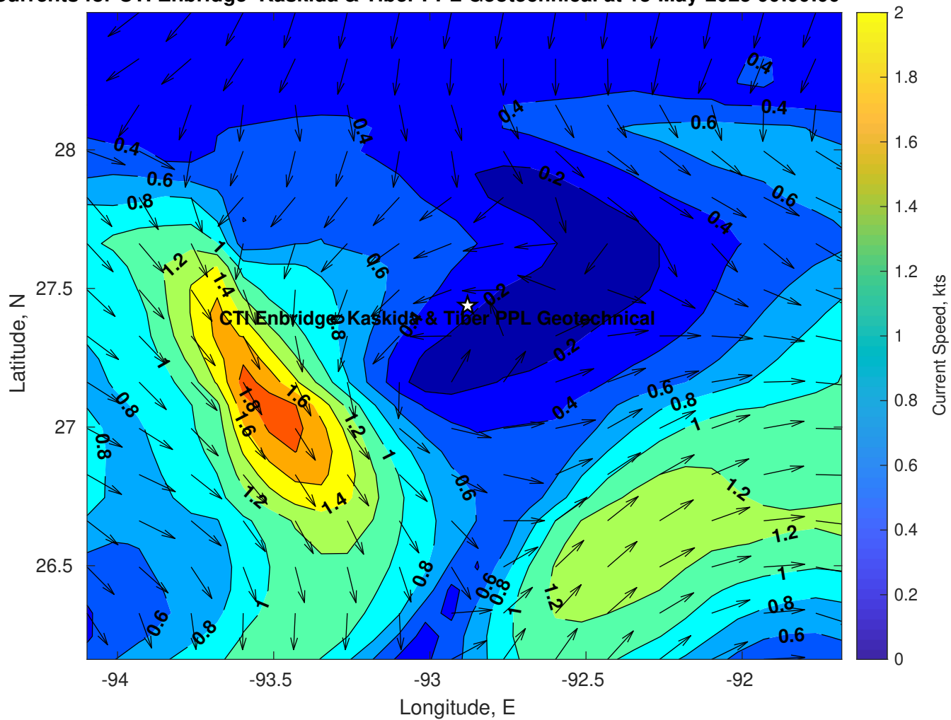
Surface Currents for CTI Enbridge Kaskida & Tiber PPL Geotechnical at 13-May-2025 00:00:00
