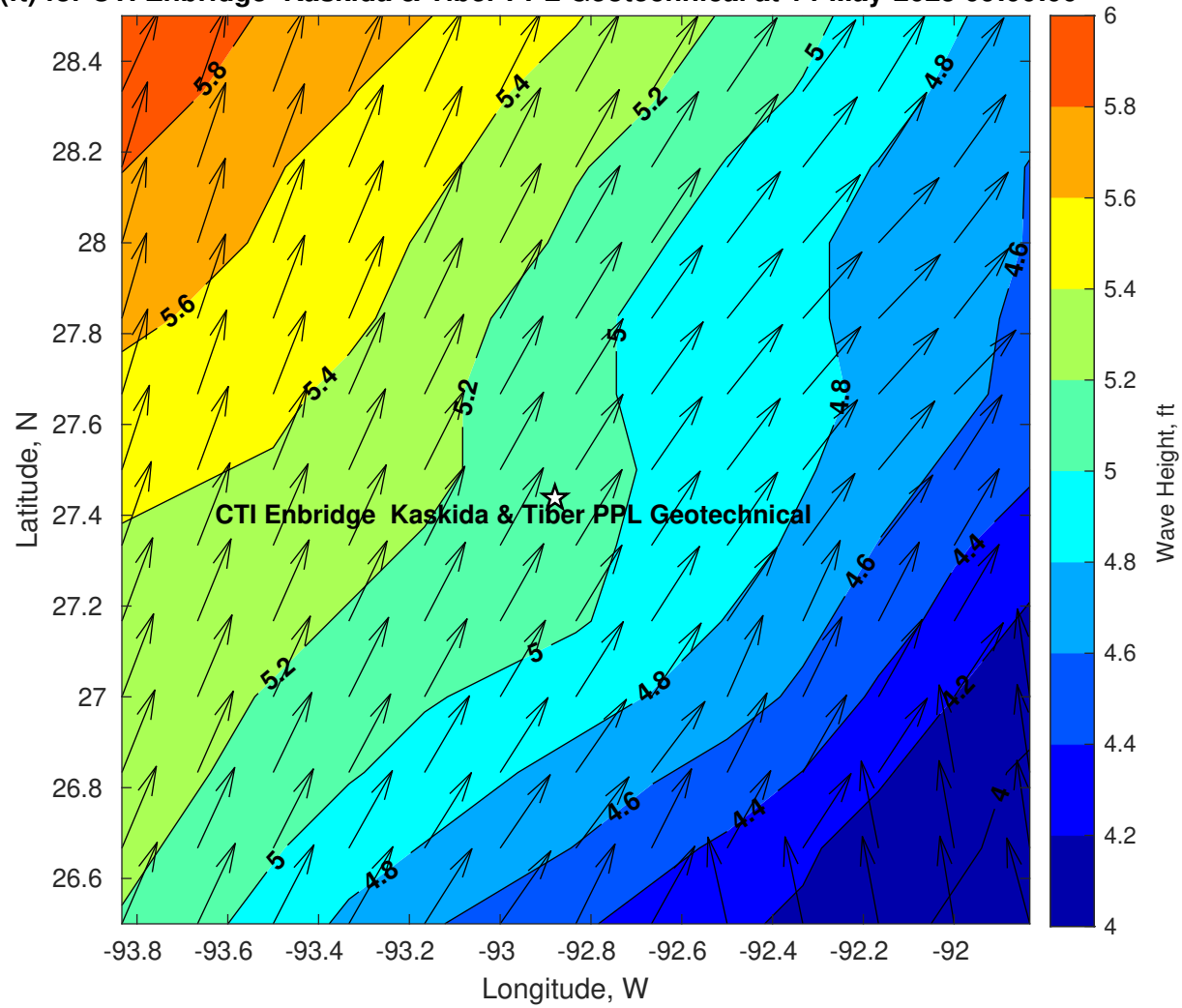
Wave Height (ft) for CTI Enbridge Kaskida & Tiber PPL Geotechnical at 14-May-2025 09:00:00
