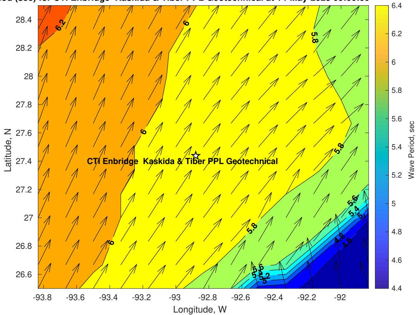
Wave Period (sec) for CTI Enbridge Kaskida & Tiber PPL Geotechnical at 14-May-2025 09:00:00
