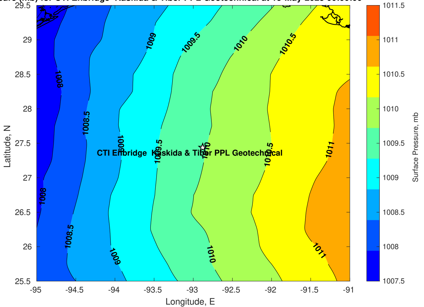
Surface Pressure (mb) for CTI Enbridge Kaskida & Tiber PPL Geotechnical at 15-May-2025 00:00:00
