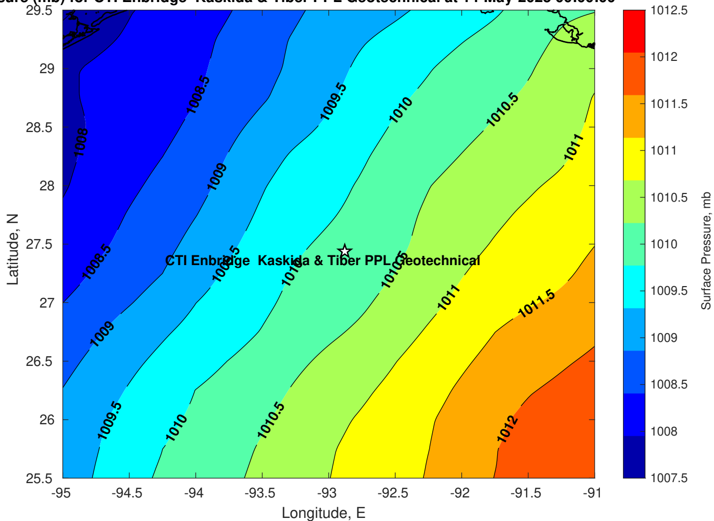
Surface Pressure (mb) for CTI Enbridge Kaskida & Tiber PPL Geotechnical at 14-May-2025 00:00:00
