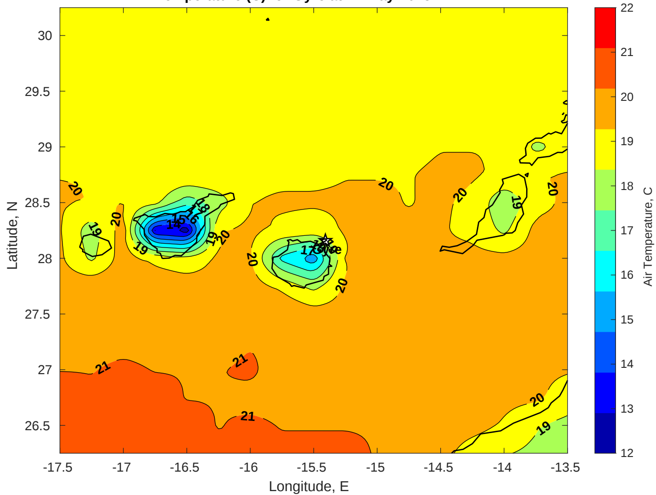
Air Temperature (C) for Gyre at 14-May-2025
