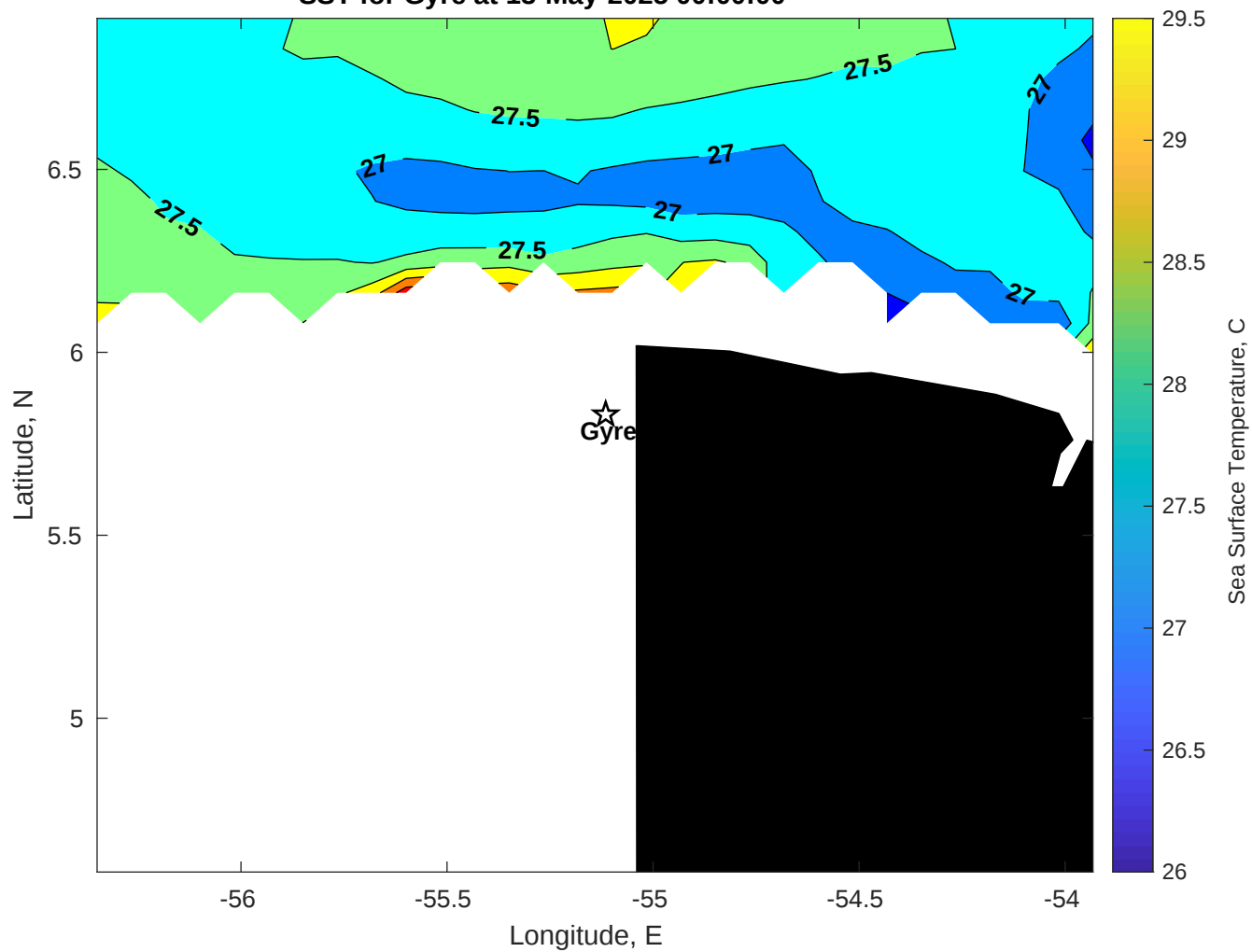
SST for Gyre at 13-May-2025 00:00:00
