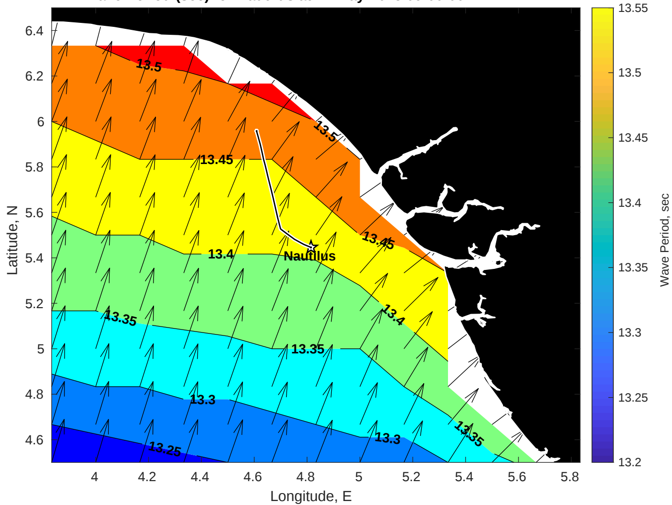
Wave Period (sec) for Nautilus at 14-May-2025 09:00:00
