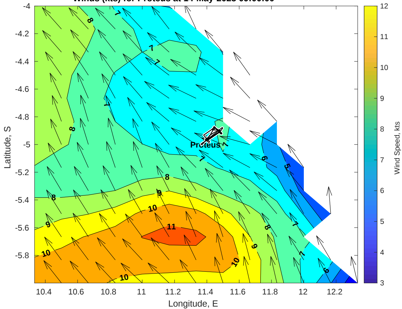
Winds (kts) for Proteus at 14-May-2025 09:00:00
