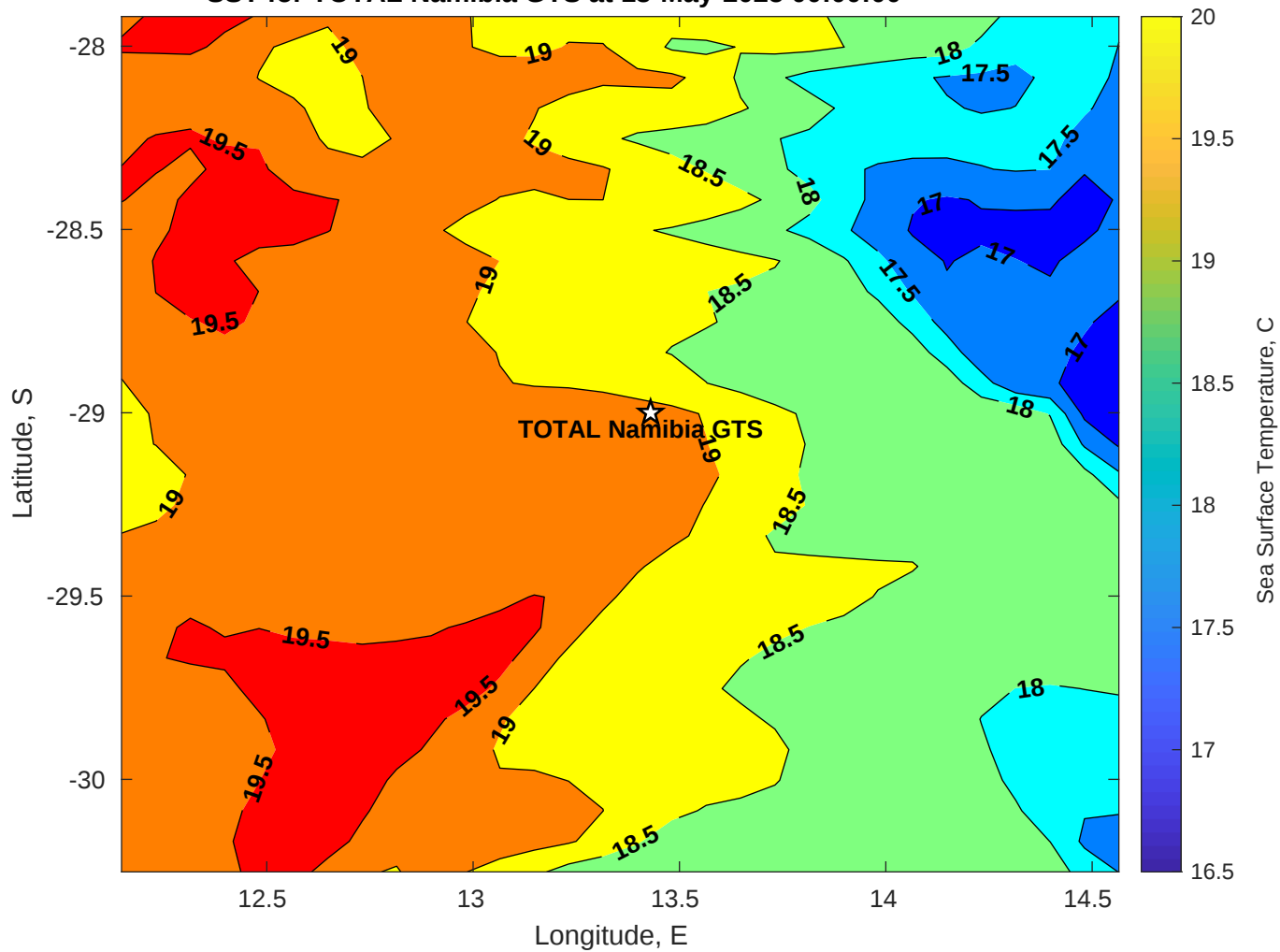
SST for TOTAL Namibia GTS at 13-May-2025 00:00:00
