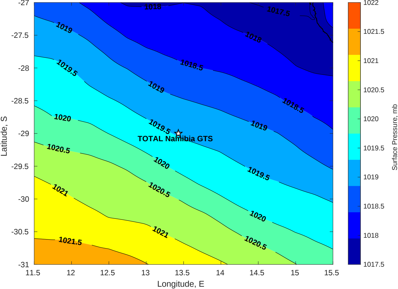
Surface Pressure (mb) for TOTAL Namibia GTS at 14-May-2025 00:00:00
