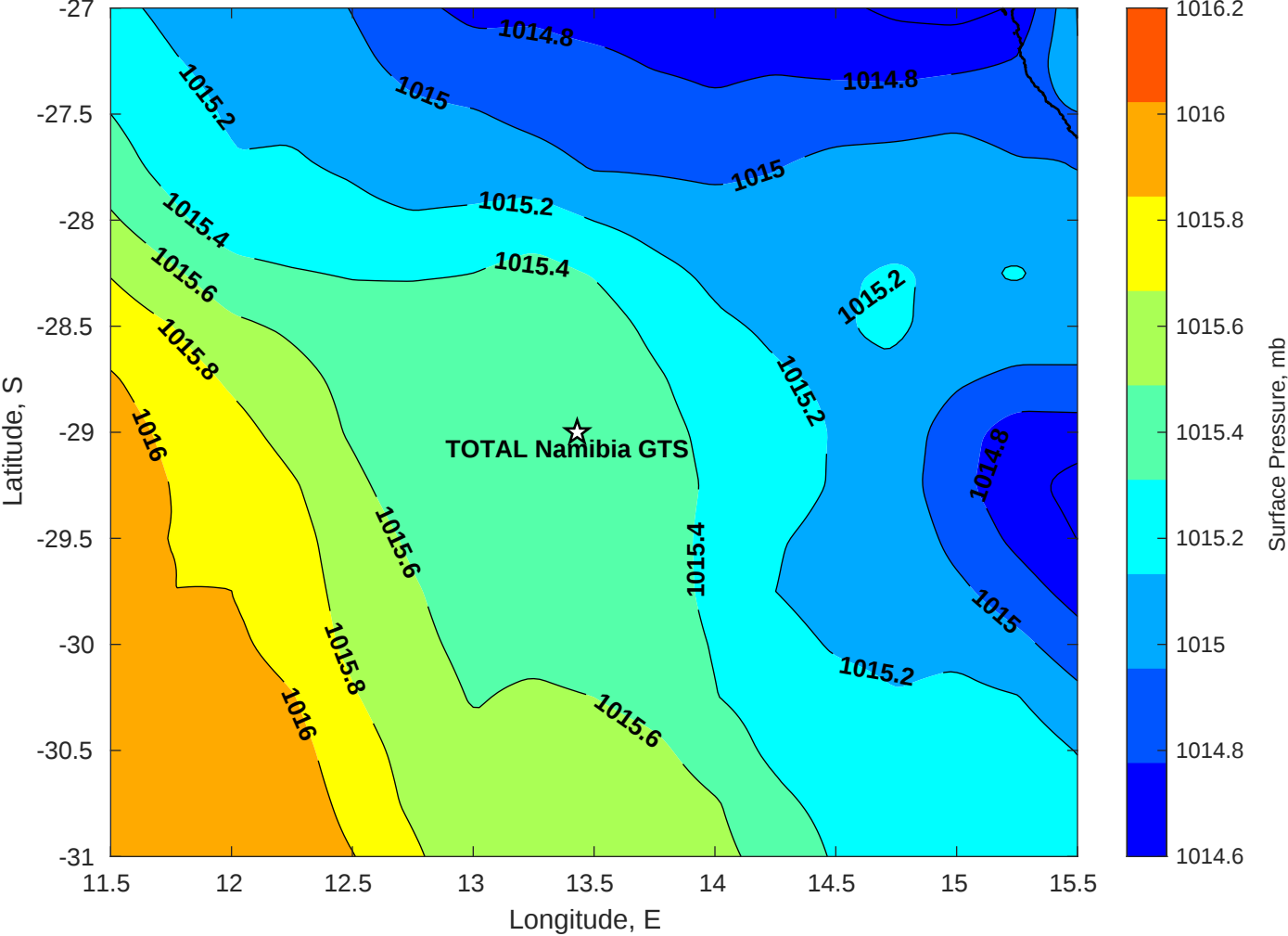
Surface Pressure (mb) for TOTAL Namibia GTS at 16-May-2025 00:00:00
