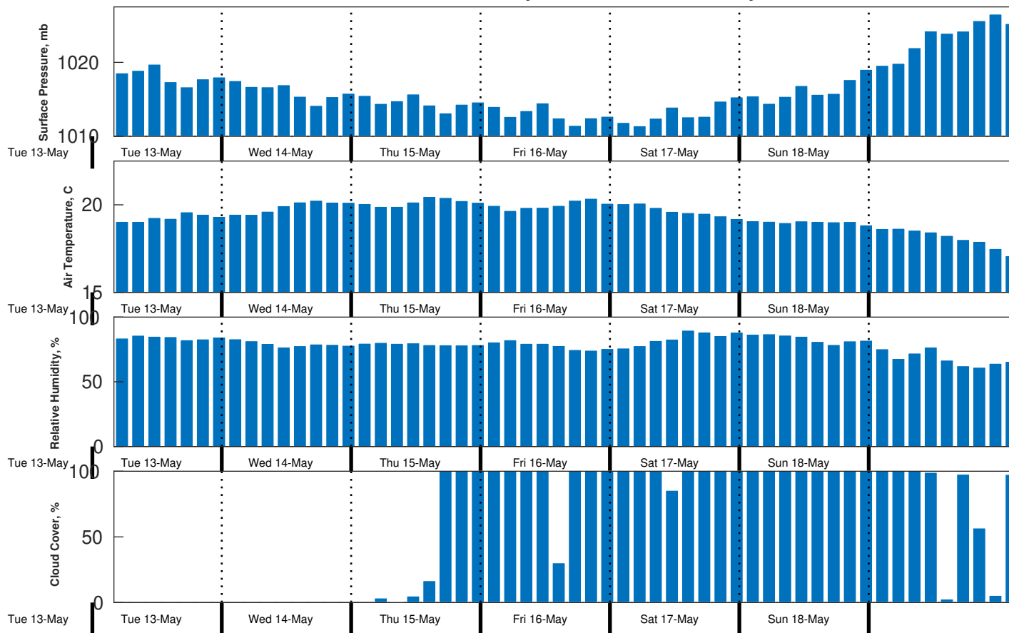
Met Forecast for TOTAL Namibia GTS from 14-May-2025 00:00:00 to 21-May-2025 00:00:00
