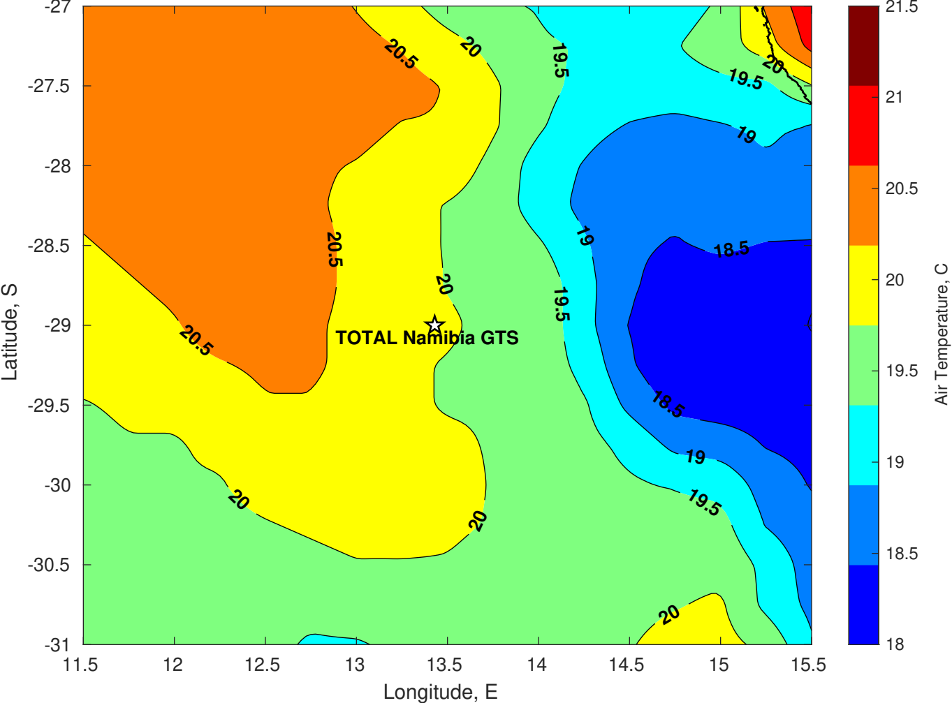
Air Temperature (C) for TOTAL Namibia GTS at 14-May-2025
