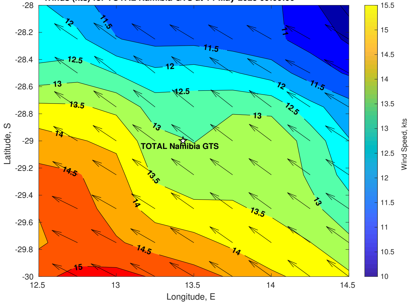
Winds (kts) for TOTAL Namibia GTS at 14-May-2025 09:00:00
