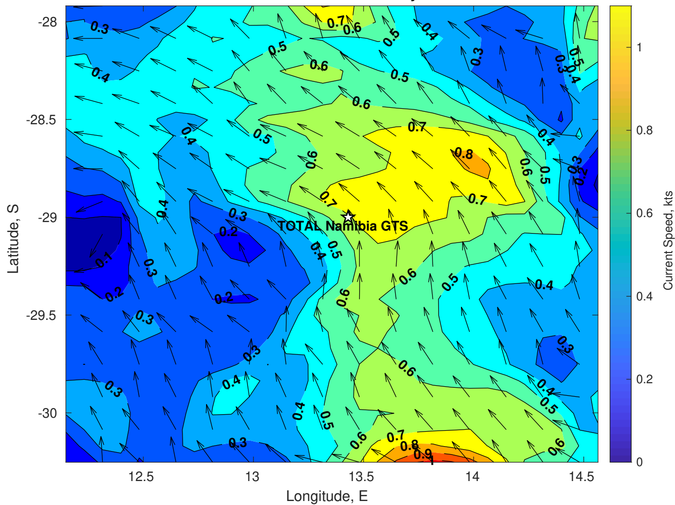
Surface Currents for TOTAL Namibia GTS at 13-May-2025 00:00:00
