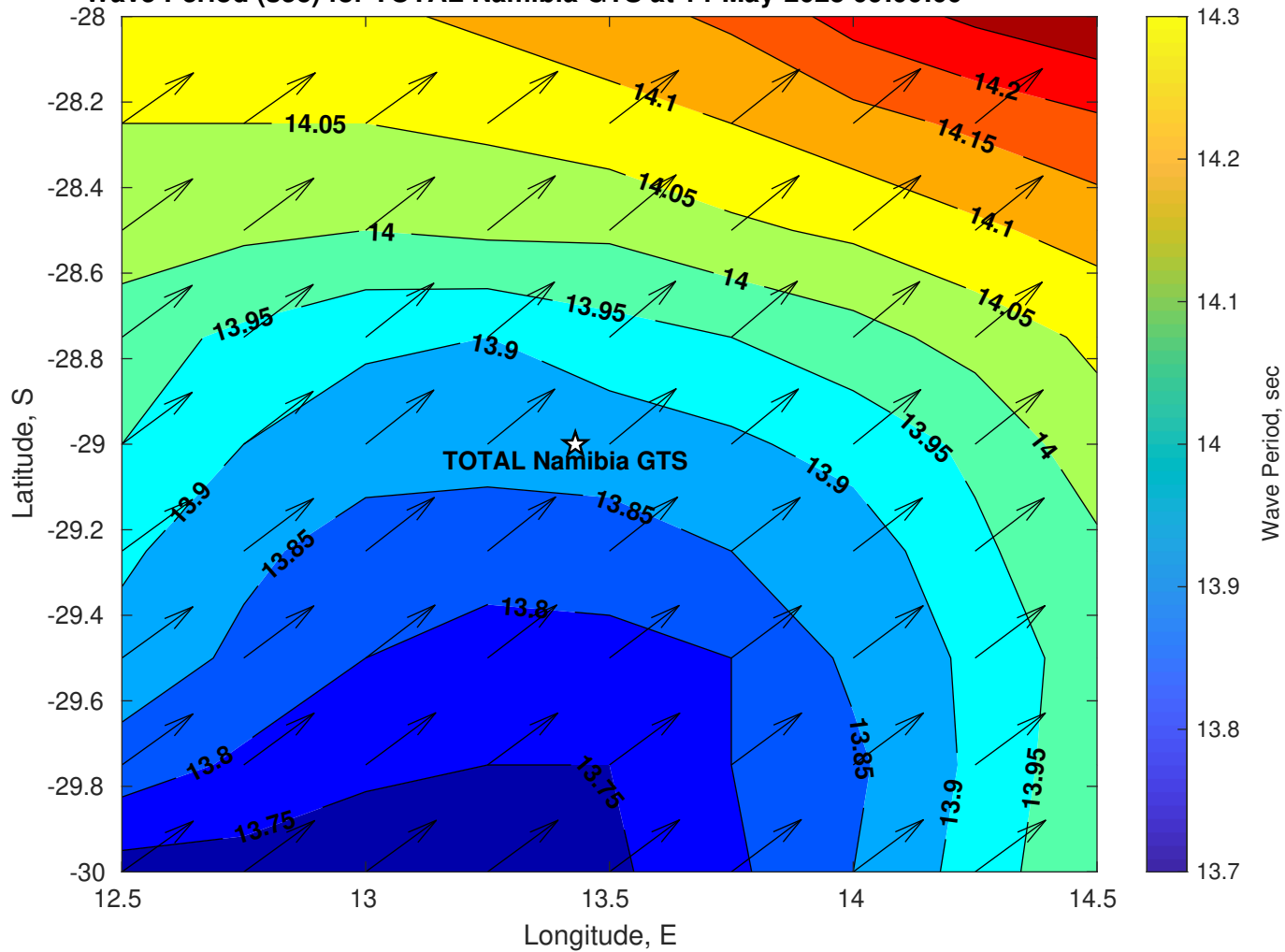
Wave Period (sec) for TOTAL Namibia GTS at 14-May-2025 09:00:00
