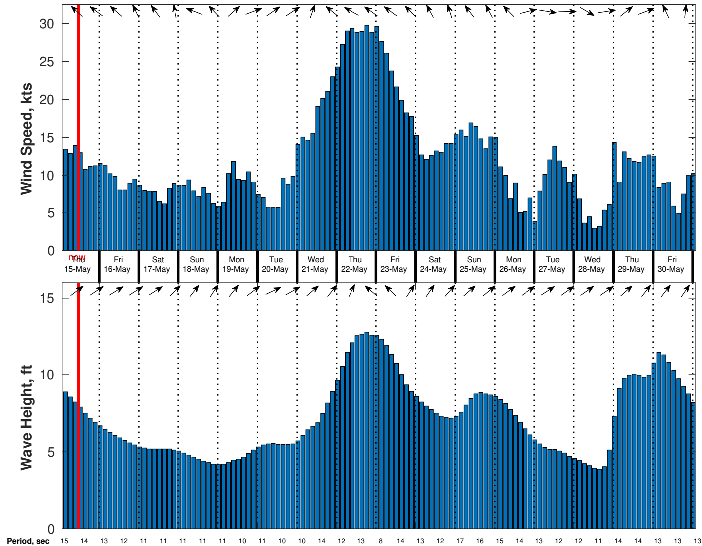
Wind & Wave Forecast for TOTAL Namibia GTS from 14-May-2025 02:00:00 to 30-May-2025 02:00:00
