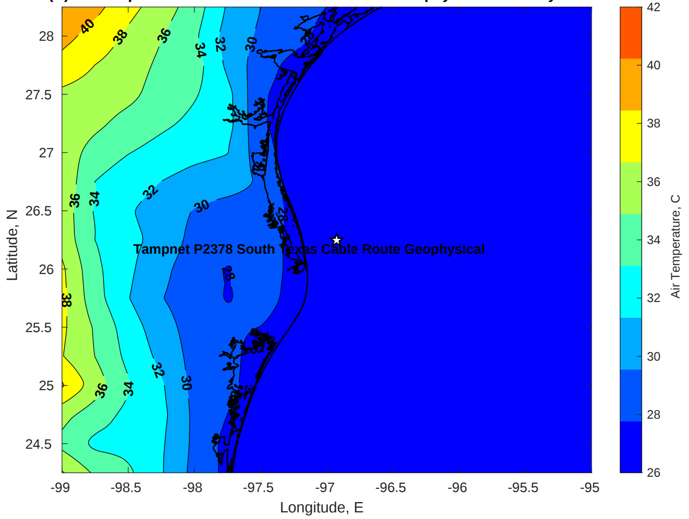
Air Temperature (C) for Tampnet P2378 South Texas Cable Route Geophysical at 14-May-2025
