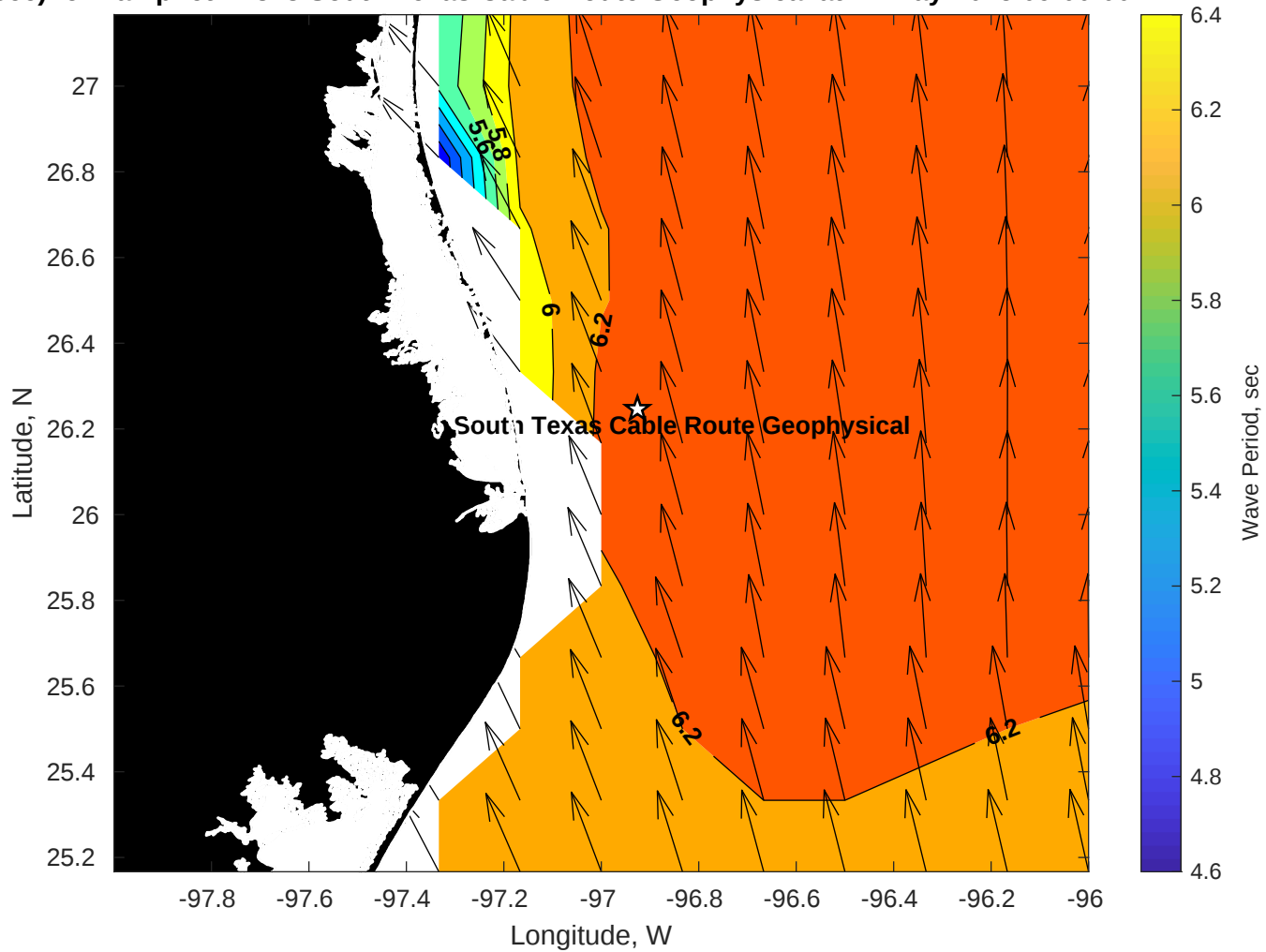
Period (sec) for Tampnet P2378 South Texas Cable Route Geophysical at 14-May-2025 09:00:00
