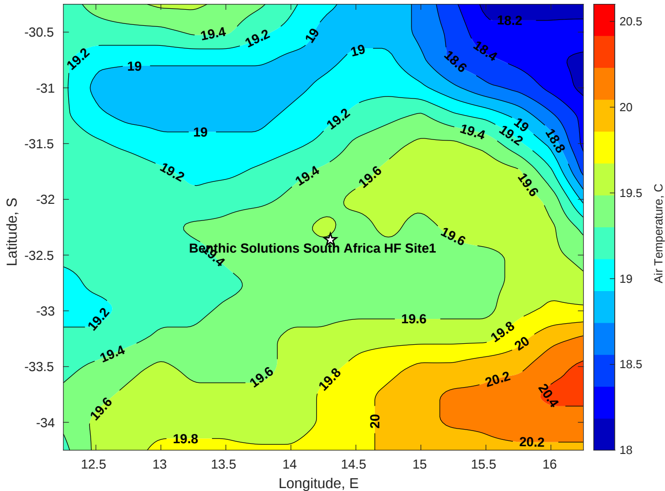
Air Temperature (C) for Benthic Solutions South Africa HF Site1 at 15-May-2025
