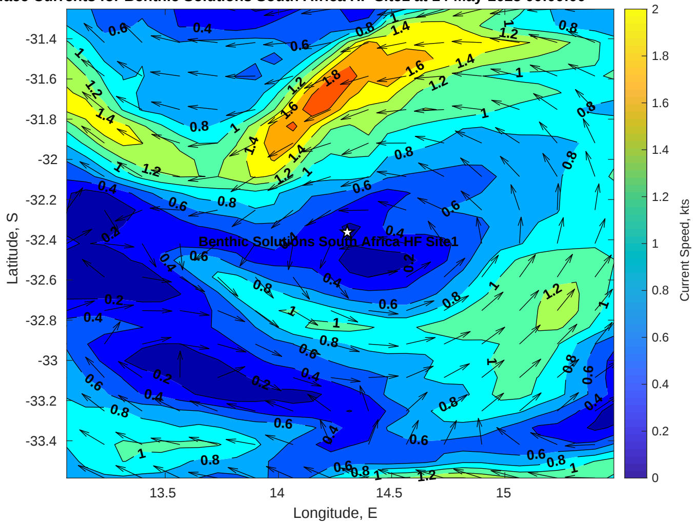
Surface Currents for Benthic Solutions South Africa HF Site1 at 14-May-2025 00:00:00
