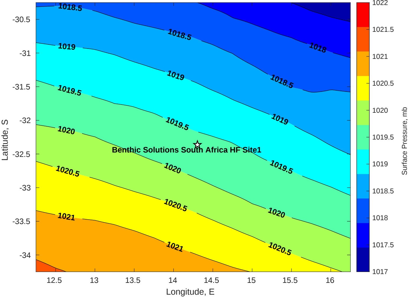
Surface Pressure (mb) for Benthic Solutions South Africa HF Site1 at 15-May-2025 00:00:00
