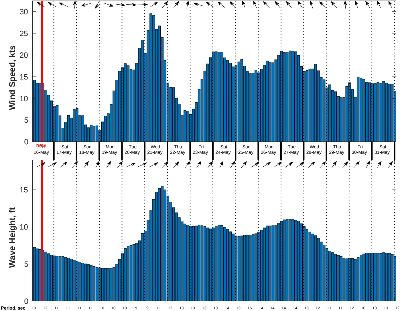
Wind & Wave Forecast for Benthic Solutions South Africa HF Site1 from 15-May-2025 02:00:00 to 31-May-2025 02:00:00
