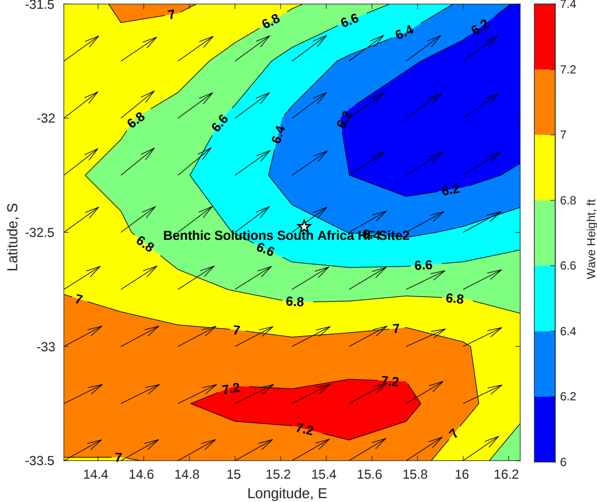
Wave Height (ft) for Benthic Solutions South Africa HF Site2 at 15-May-2025 09:00:00
