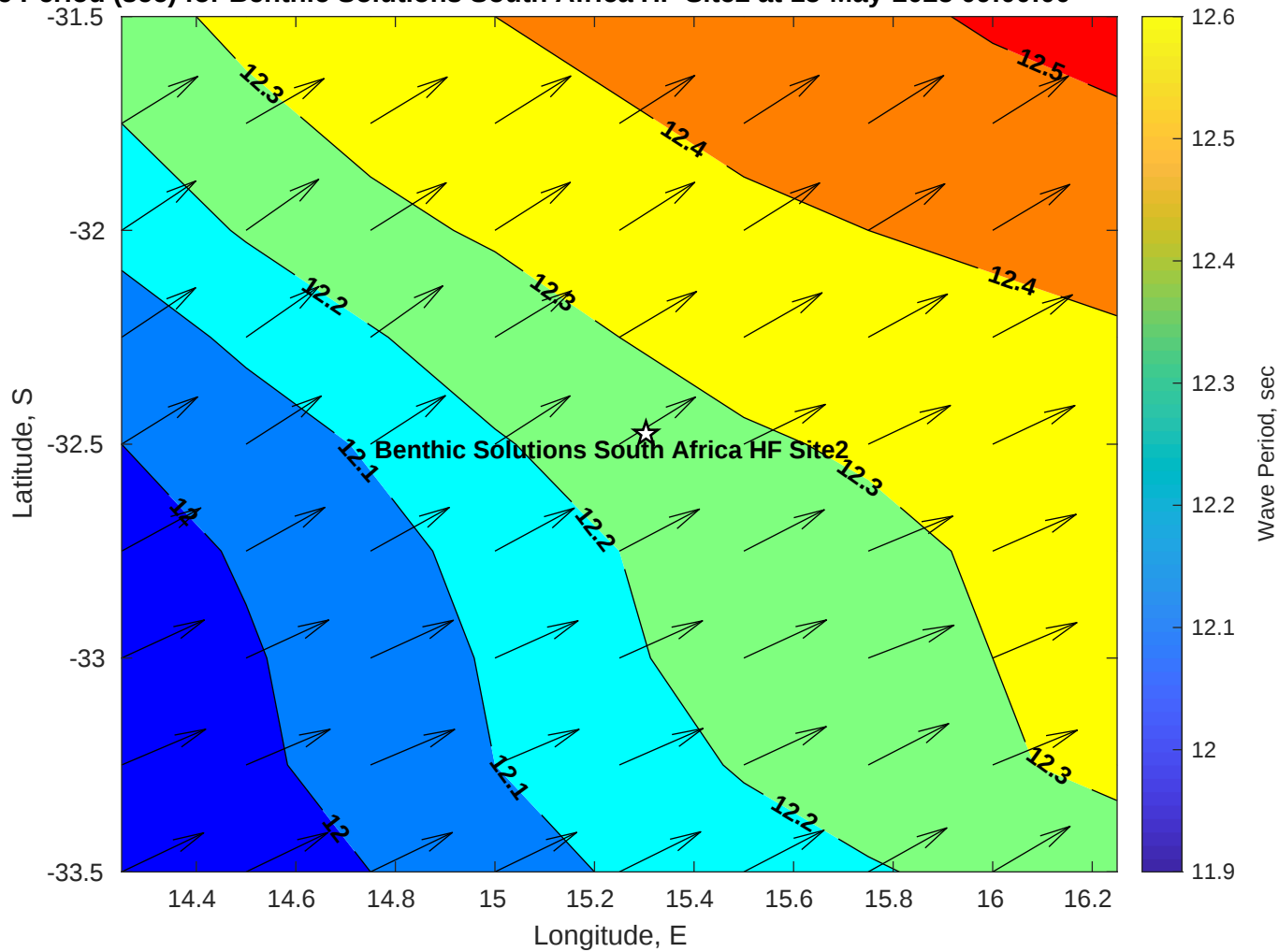
Wave Period (sec) for Benthic Solutions South Africa HF Site2 at 15-May-2025 09:00:00
