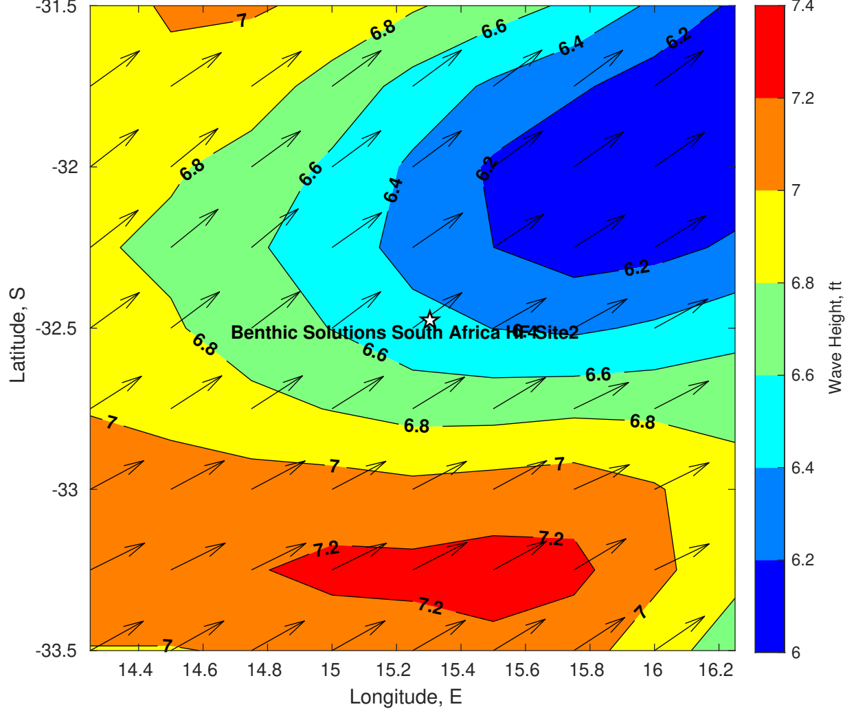
Wave Height (ft) for Benthic Solutions South Africa HF Site2 at 15-May-2025 09:00:00
