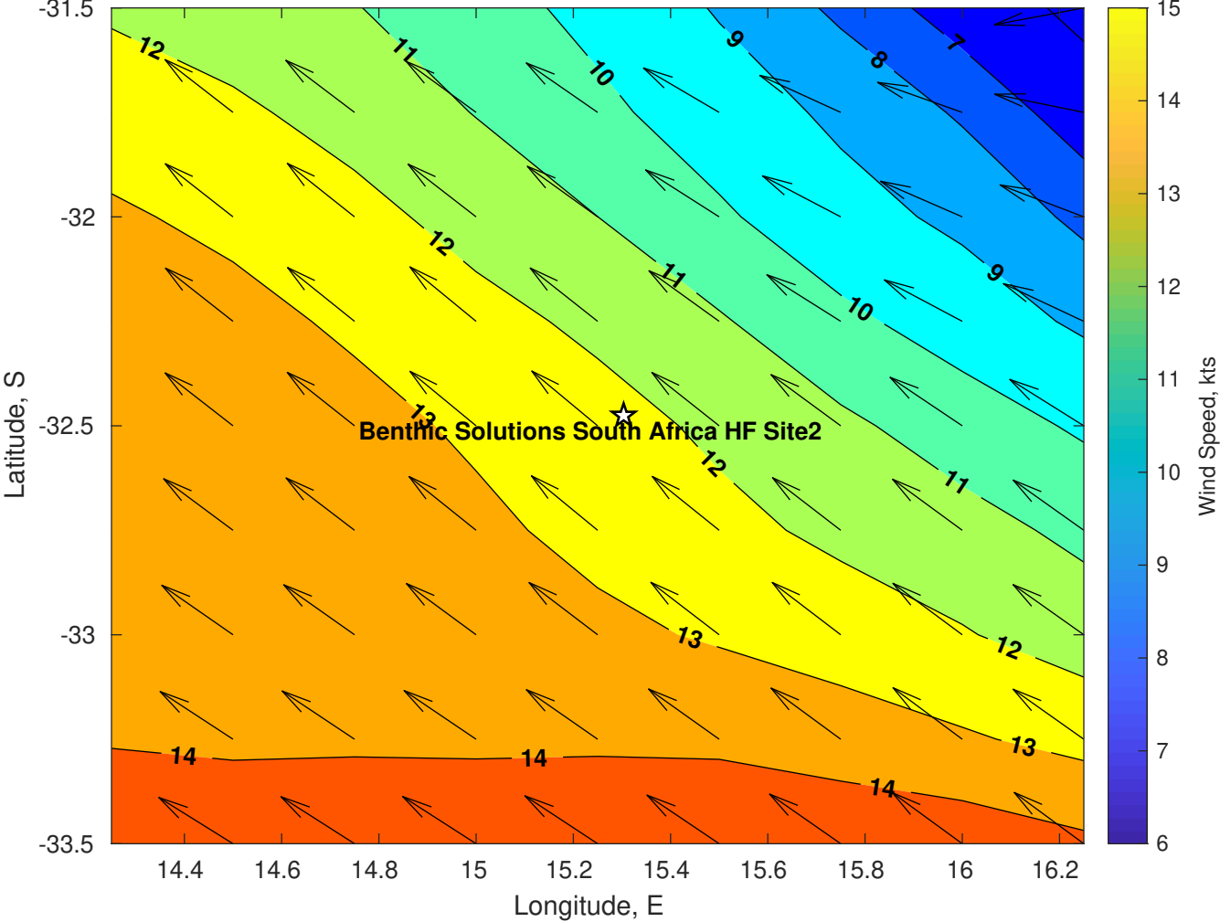
Winds (kts) for Benthic Solutions South Africa HF Site2 at 15-May-2025 09:00:00
