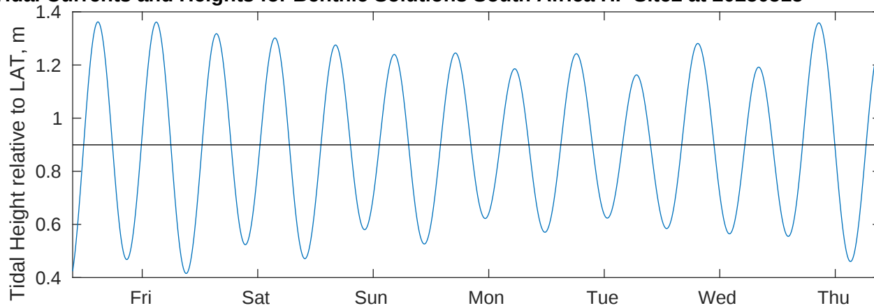
Tidal Currents and Heights for Benthic Solutions South Africa HF Site2 at 20250515
