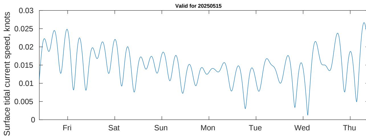
Tidal Currents and Heights for Benthic Solutions South Africa HF Site2 at 20250515
