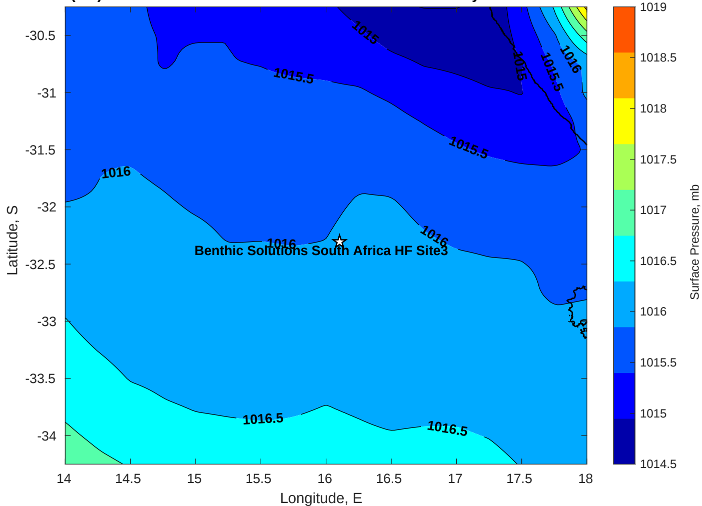
Surface Pressure (mb) for Benthic Solutions South Africa HF Site3 at 16-May-2025 00:00:00
