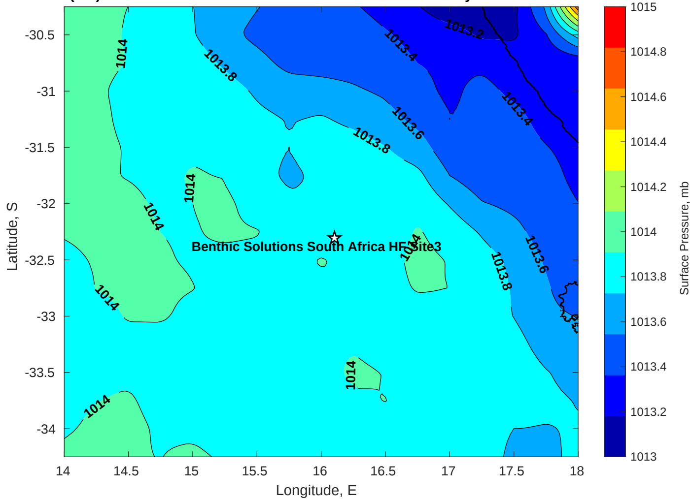
Surface Pressure (mb) for Benthic Solutions South Africa HF Site3 at 17-May-2025 00:00:00
