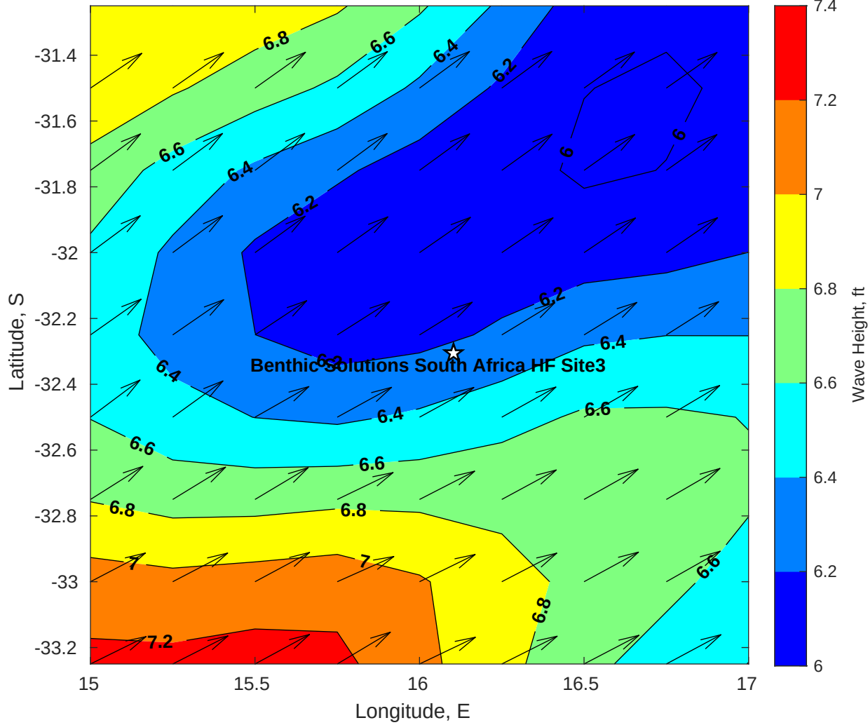
Wave Height (ft) for Benthic Solutions South Africa HF Site3 at 15-May-2025 09:00:00
